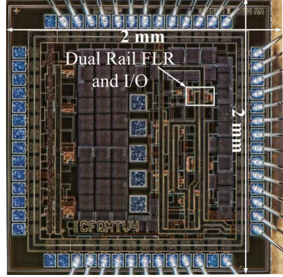
Fig. 9. Microphotograph of the fabricated testchip of the proposed multi-power rail power pad and I/O in a 0.18 \mu m technology.
