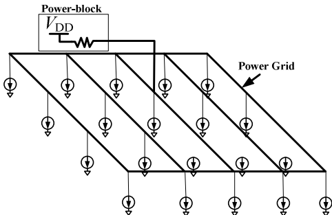
Fig. 4. Simplified worst case model of the WaferIC power grid with an equivalent resistance of 250 m \Omega in series with each active circuit (modeled as current source).
