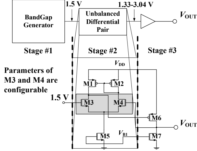
Figure 5.3 Unbalanced differential pair using a single 1.5 V voltage reference to generate 246 output voltages at 10 mV step-intervals, ranging from 1.33 to 3.04 V [17].
