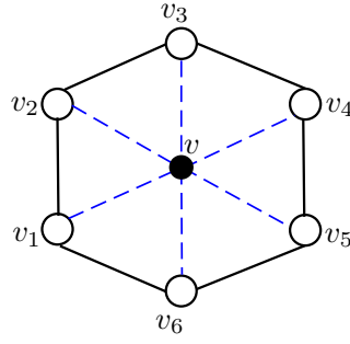
Figure 4.1 Example of wheel with q = 6 .
