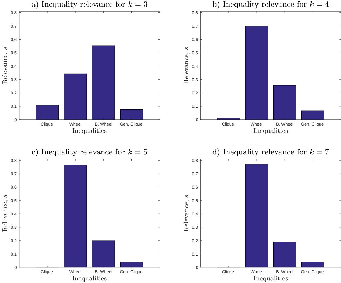
Figure 4.6 Relevance of the inequalities for all instances.
