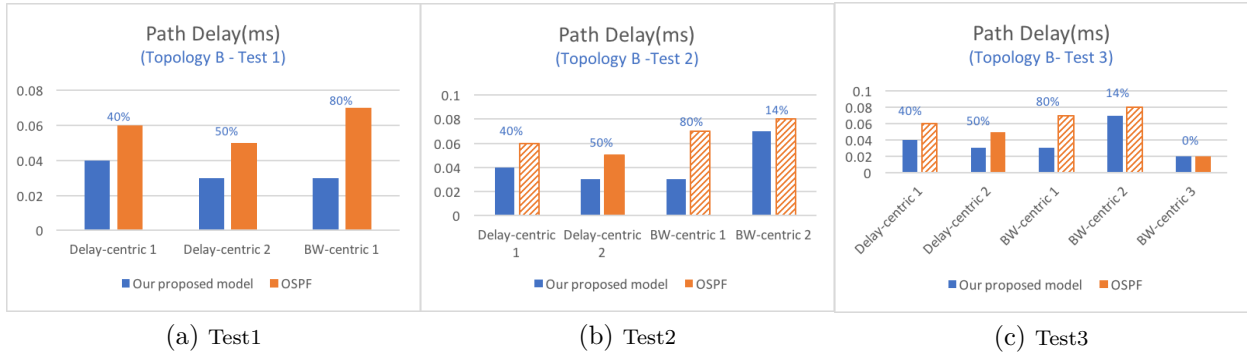
Figure 5.10 Path delay result - Topology B
