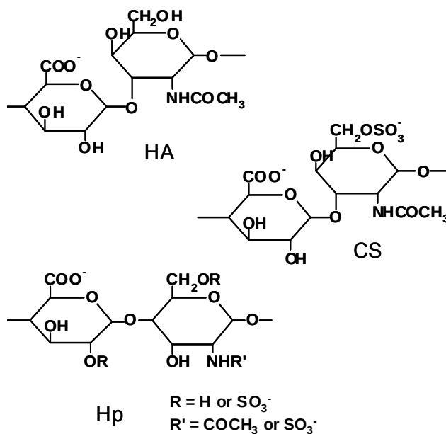
Figure A.2.1. Structure of Hyaluronan (HA), Chondroitin-6-Sulfate (CS), and Heparin (Hp) disaccharides.
