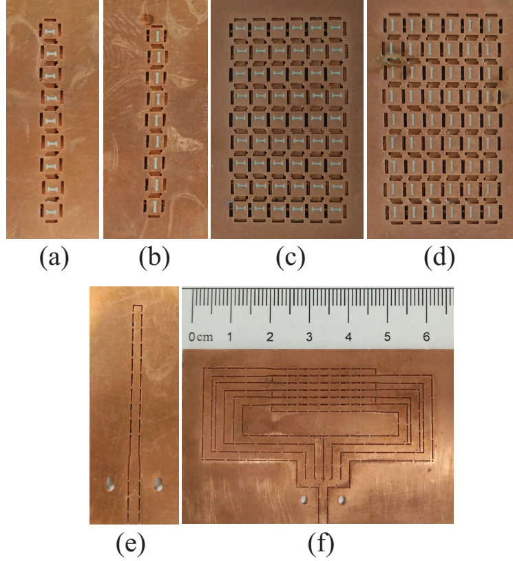
Figure 4.7 Fabricated prototypes, (a) 1D X-pol radiation slots, (b) 1D Y-pol radiation slots, (c) 2D X-pol radiation slots, (d) 2D Y-pol radiation slots, (e) 1D feed network for both polarizations, (f) 2D feed network for both polarizations.
