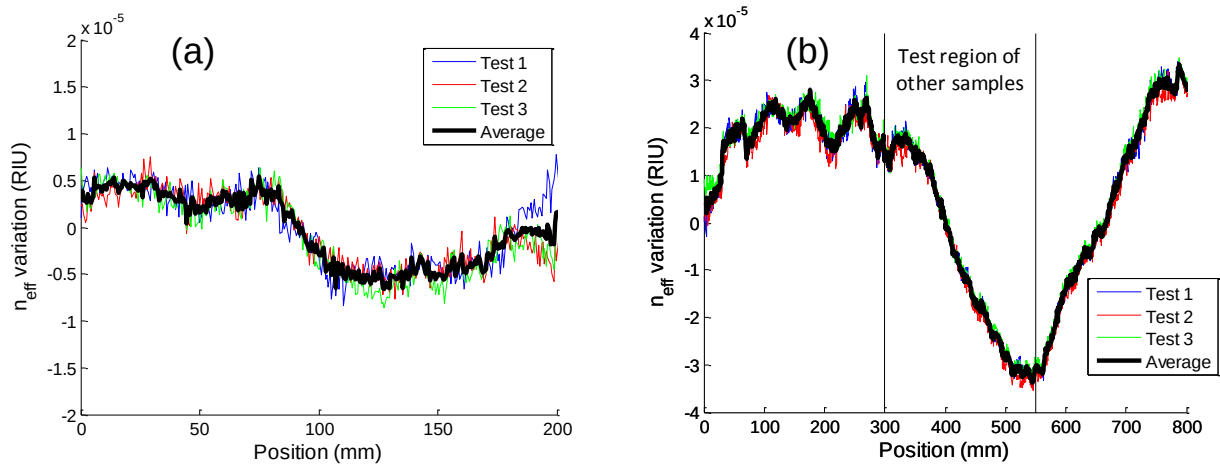
Figure 5.4: Characterization of a small-core, high NA fiber and non-PM fiber (SM2). (a) and (b) show two different fiber samples, (b) of long length. The thin lines are the 3 tests, while the tick like is the average of the 3. Note, the scale of \Delta n_{\text{eff}} in (b) is twice the scale of other figures.
