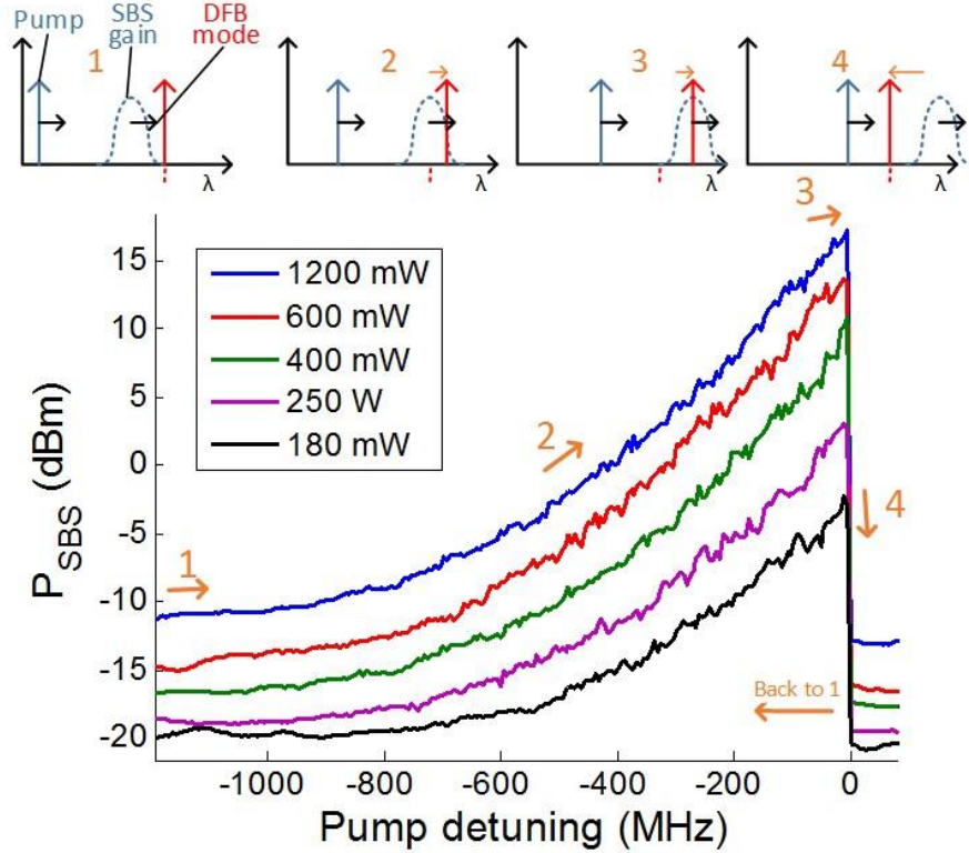
Figure 4.3: SBS generated power as a function of pump detuning and power. The pump is detuned as shown in the upper inset (by approaching the DFB mode from shorter wavelengths). The SBS gain, moving with the pump, pushes the DFB mode (state 1, 2) until the maximum is reached (state 3). The mode then “recoils” back to its original position once the maximum gain is exceeded. To recover SBS, the pump must be detuned to a shorter wavelength (state 1) to re-initiate SBS generation.
