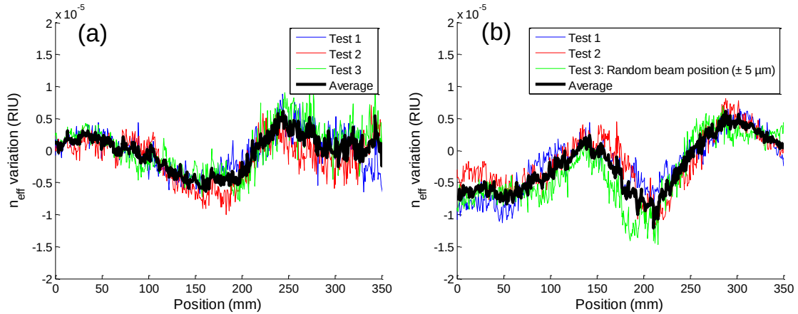
Figure 5.5: Characterization of a 6μm mode field diameter PM fiber (PM2). (a) and (b) show two different fiber samples. 3 tests are shown with the average. The 3rd test in (b) was done by including \pm 5 \mu\text{m} random displacement in the beam over \sim 5 cm range.
