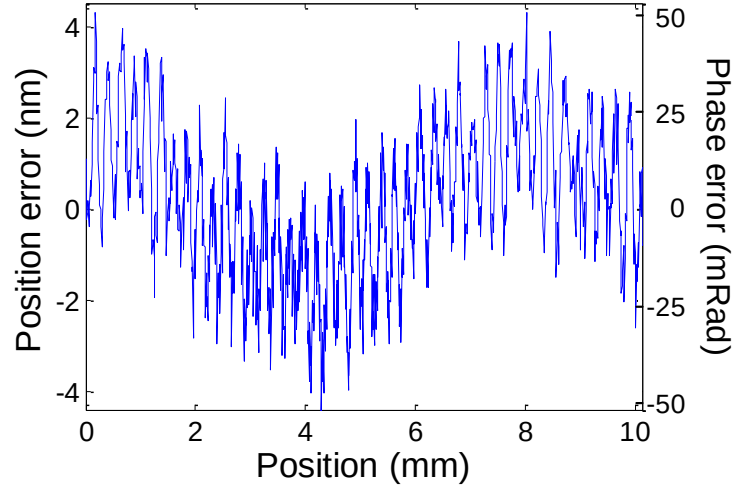
Figure 8.4: Position error noise, hence phase error noise, measured by the stage. The measured data was spatially averaged over the illumination spot size of 120\text{ }\mu\text{m} .
