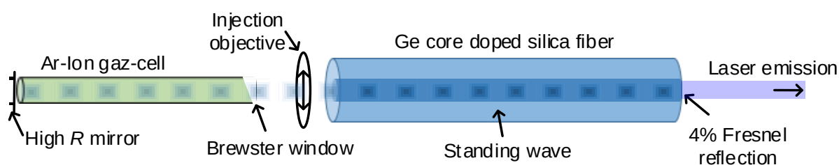
Figure 1.1: Hill et al.'s experiment discovering photosensitivity and how to make FBGs using an Ar-ion laser. A Fresnel reflection caused a standing wave in a Ge-doped silica fiber, which in turn wrote a permanent grating in the fiber through photosensitivity.
