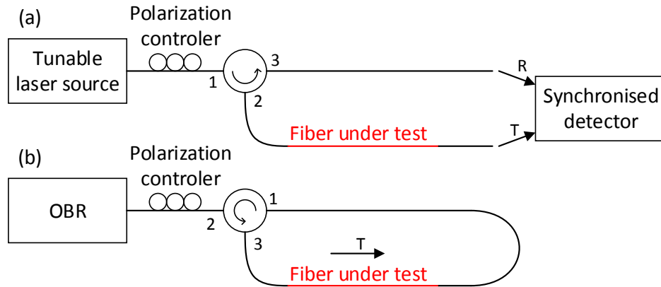
Figure 3.5: Measurement method
