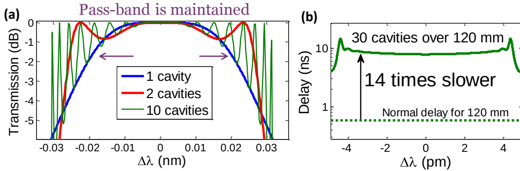
Figure 2.13: Simulation and design of broad-band superimposed CFBG cavity arrays. (a) Transmission spectrum of 1 to 10 cavities to show how the pass-band is relatively maintained. (b) Delay with wavelength of a 30 superimposed CFBG cavity array.
