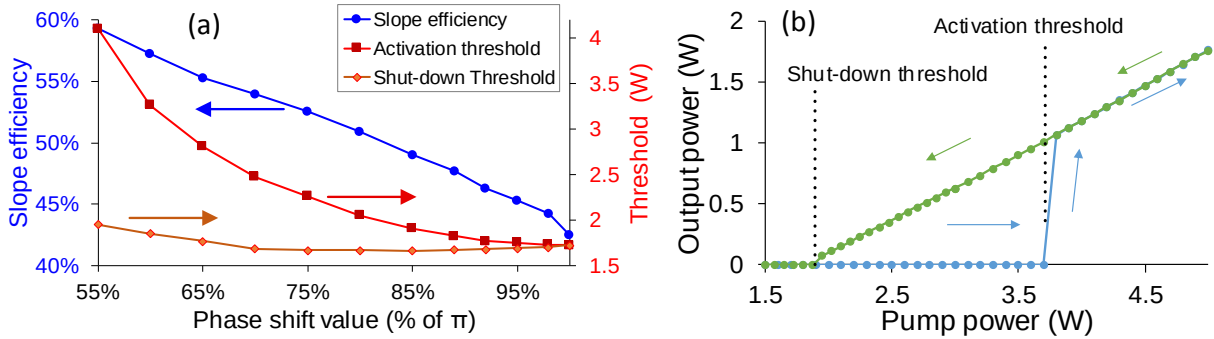
Figure 7.5: Effect of phase-shift value. (a) The activation threshold (when increasing the pump from 0 W initially), shut-down threshold (when decreasing the pump after achieving lasing state) and slope efficiency are shown with varying phase-shift values (b) An example of activation/shut-down hysteresis is shown with a phase shift of 0.6\pi . FBGs are 300 mm long with a phase shift at -8% from center. \kappa_{ac} is 40 m -1 and the loss is 0.03 dB/m.
