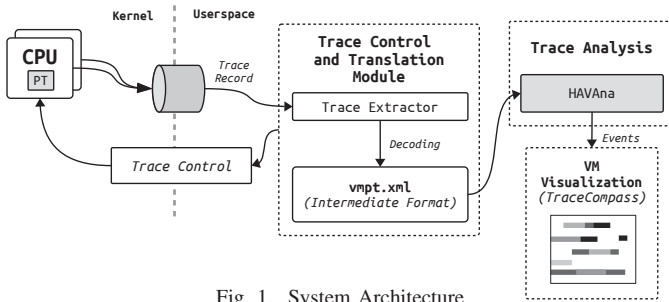
Fig. 1. System Architecture
