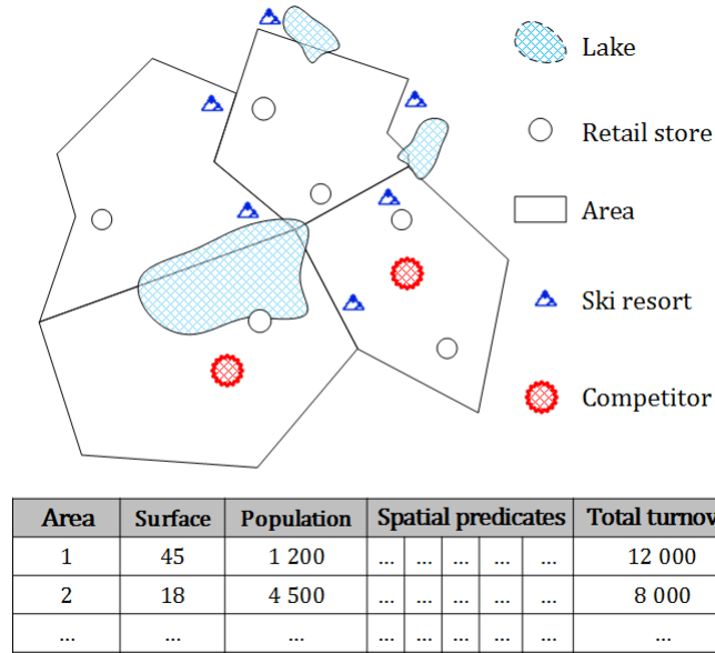
Figure 5.5 Data Integration
