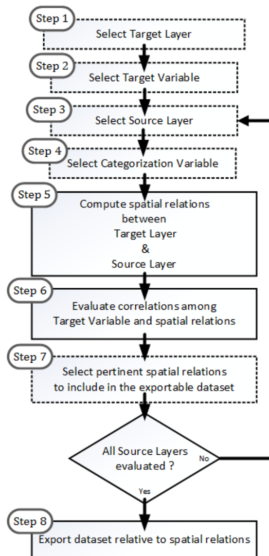
Figure 5.8 Pre-Processing Steps
