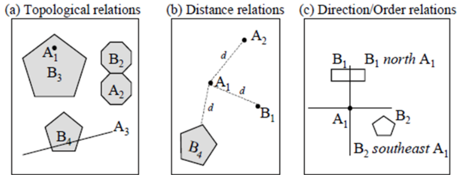
Figure 5.1 Spatial Relations ([18])
