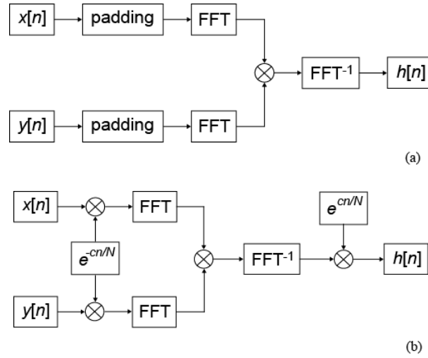
Figure B.3 : Block diagrams of the operations involved in the calculation of the linear convolution with (a) the zero-padding method and b) the NLT method. The process shown in (b) produces half of the 2N values of the linear convolution
