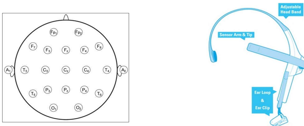
Figure 2-2 : a) A 19 electrodes positioning map based on the 10-20 system of a medical grade headset, b) A single Fp1 electrode low cost headset
