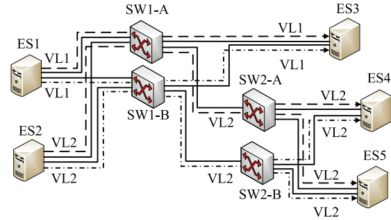
Fig. 1: An example of AFDX network architecture.
