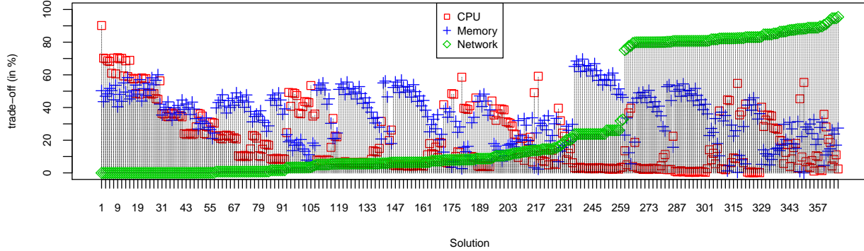
Figure 9.6: Trade-off (in %) for CPU, memory, and network usages of each optimal solution found by APOA for the emerging market context of use.
