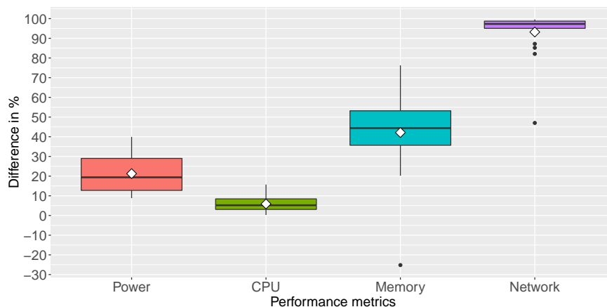
Figure 8.1: Performance metric differences for ads-supported and paid apps. The lines in the boxes indicate the minimum value, lower quartile, median, upper quartile, and maximum values. The “ \diamond ” symbols represent the average value.
