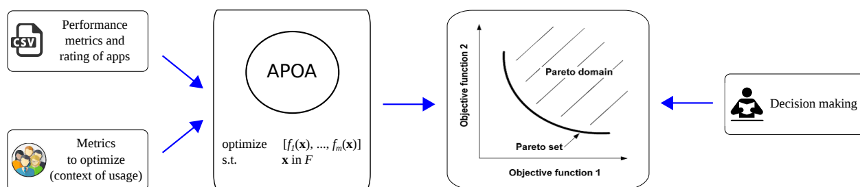
Figure 9.1: APOA conceptual sequence of steps. It uses as input a set of metrics to optimize and metric values for a set of apps belonging to different categories. It solves an optimization problem and it generates, as output, a Pareto optimal front. Each solution in the Pareto optimal front represents an optimal set of apps. Over the resulting Pareto optimal front the user selects the most preferred solution.
