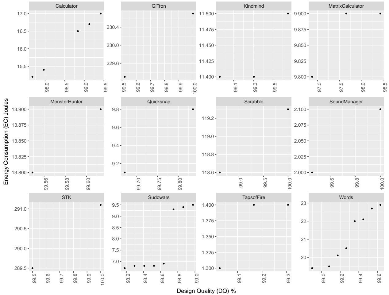
Figure 5.4: Pareto front of apps with more than one non-dominated solution found by EARMO for the case study. Each point represents a solution (refactoring sequence) with their corresponding values, design quality ( x -axis) and energy consumption ( y -axis). The most attractive solutions are located in the bottom right of each plot, because they maximize design quality while minimizing energy consumption.
