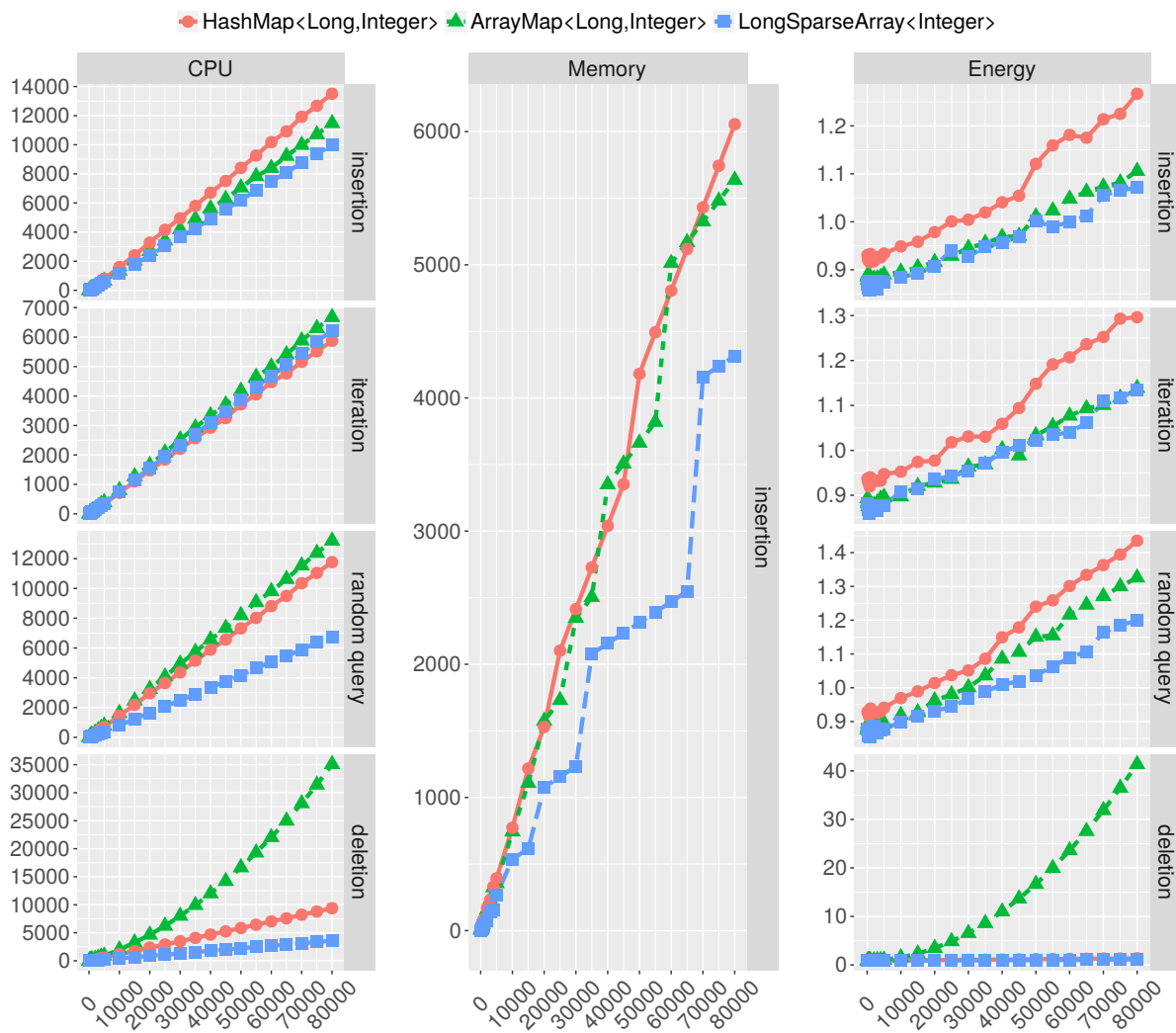
Figure 6.6: Performance metrics of map implementations using long keys and integer values, by map-related operation and data size.
