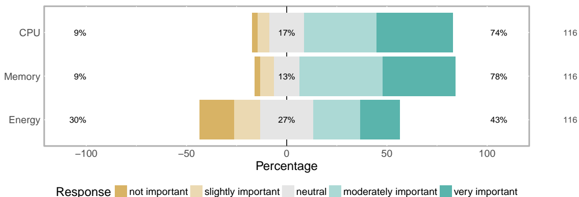
Figure 6.4: Participants’ responses about importance of performance metrics when choosing a map implementation.
