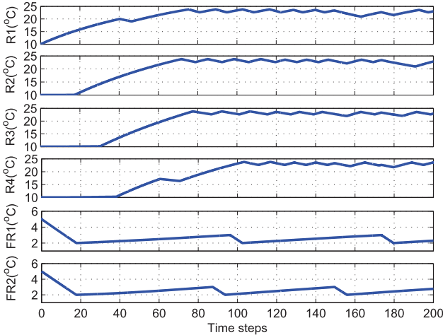
Fig. 7. Room and refrigerator temperatures using Algorithm 1.
