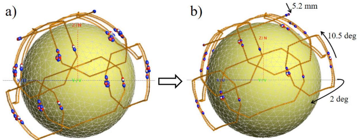
Figure 4.8 Simulated array before and after geometrical decoupling.
