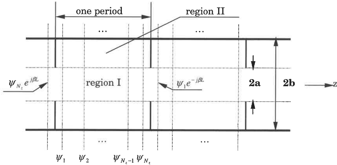
Figure 6.1 Discretization lines for a periodic cylindrical structure
