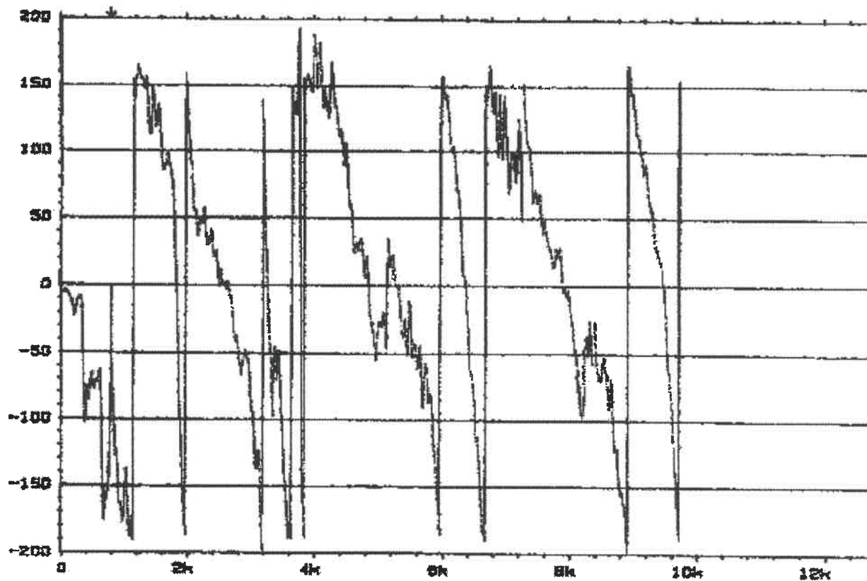
Figure A.6 The relative phase difference between the microphones at frequency from 0 to 12.8 kHz
