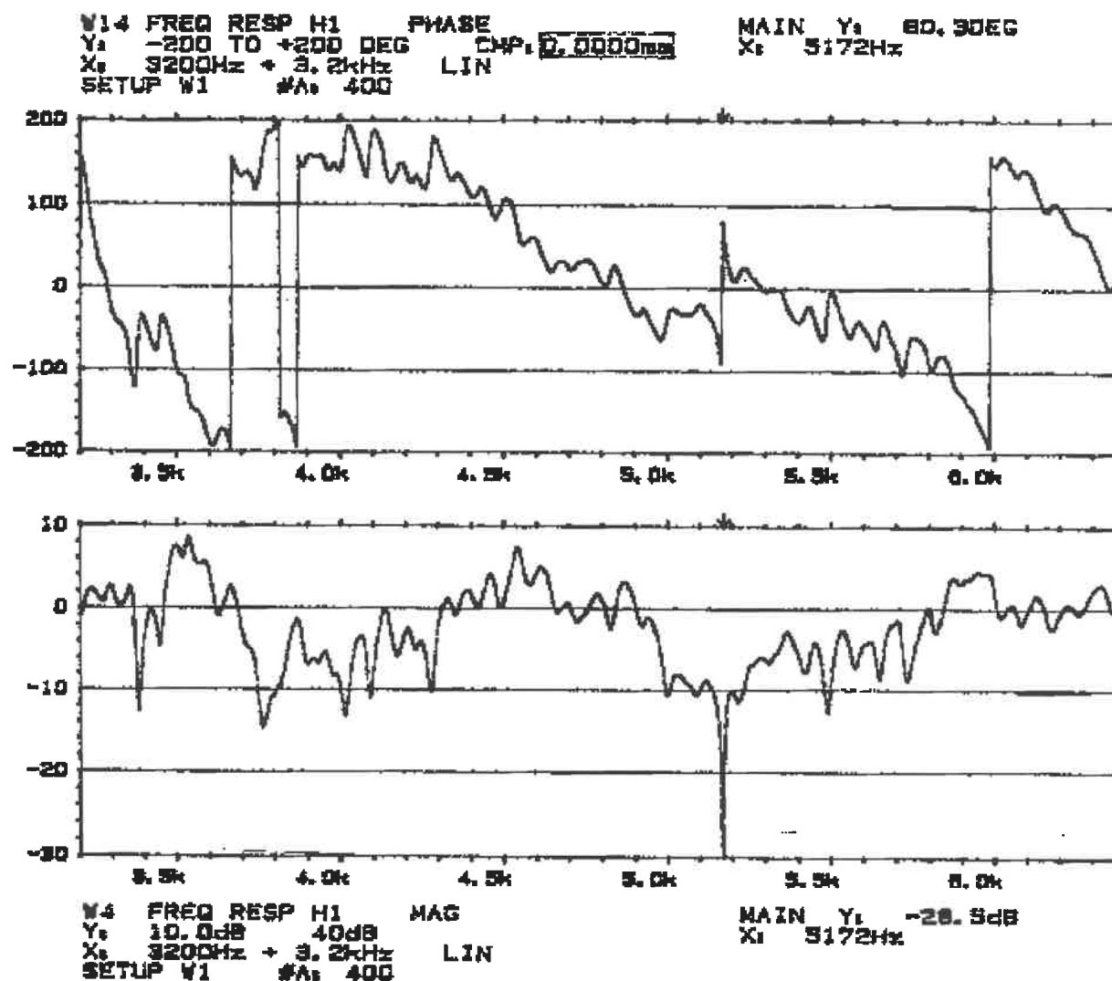
Figure A.4 The relative sound level and phase difference between the microphones at frequency from 3.2 to 6.4 kHz
