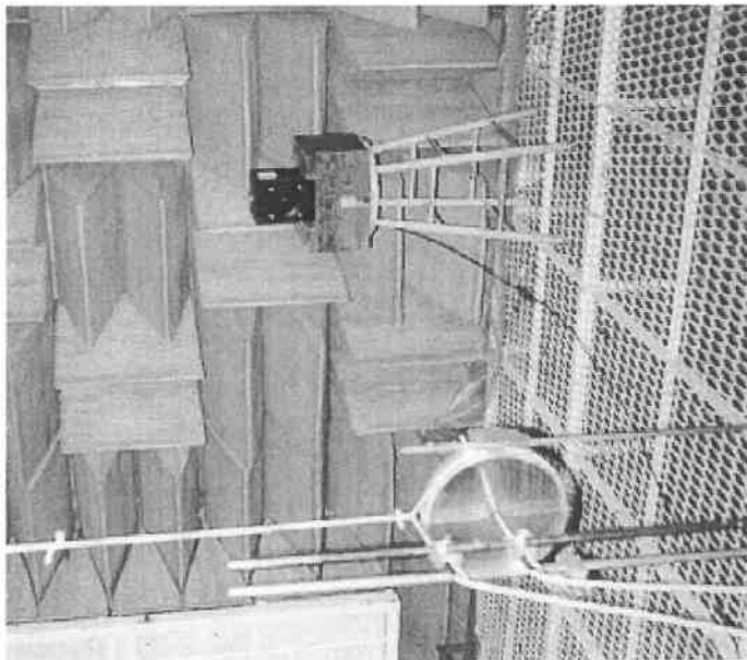
Figure B.1 The arrangement from source to receiver.
