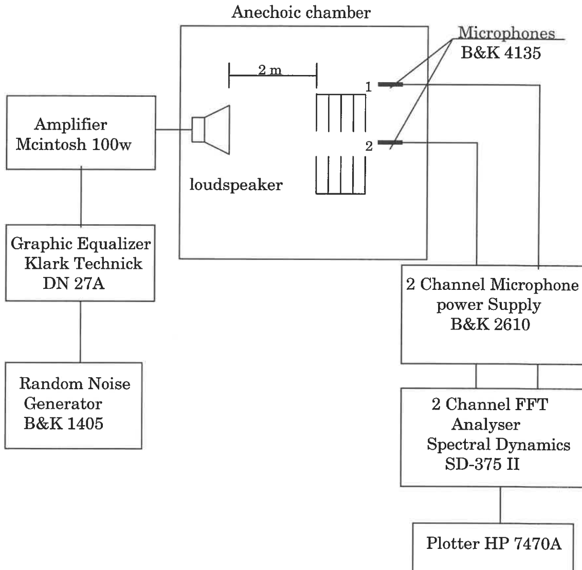
Figure 6.2 Block diagram of the measurement system
