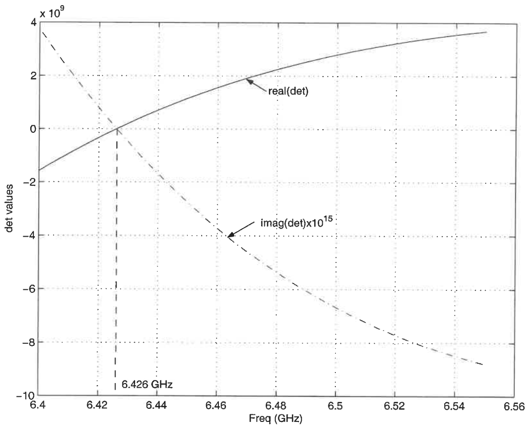
Figure 3.2a Resonant frequency of \text{TE}_{011} mode for Case A by using 2D CMoL and by calculating the determinant
