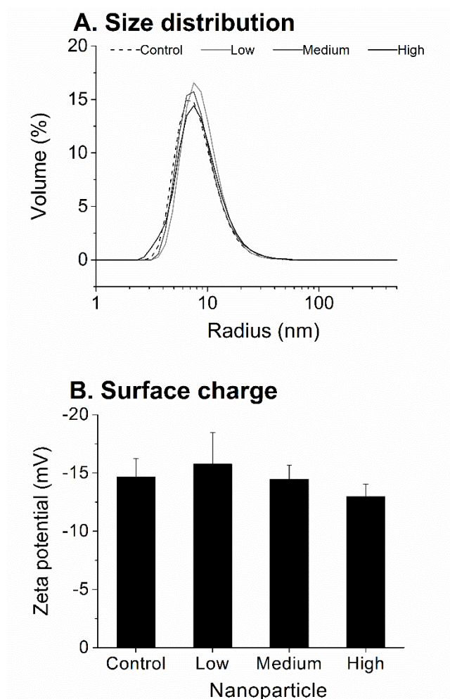
Figure annex-5 : DLS measurements of CMD/PEI polyelectrolyte complexes (PECs) bearing varying E5 surface densities (Low, Medium and High).
