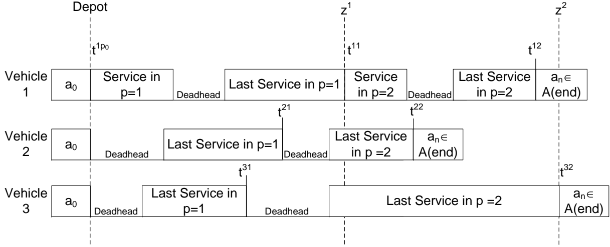
Figure 4.1 Schematic representation of the routes.
