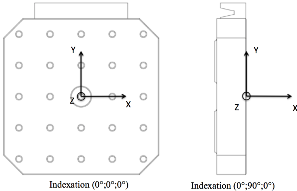
Figure 4.12 : R1 system when the machine axis positions are x=b=c=0 . The frame does not move with the table translation in X or rotation around B or C.
