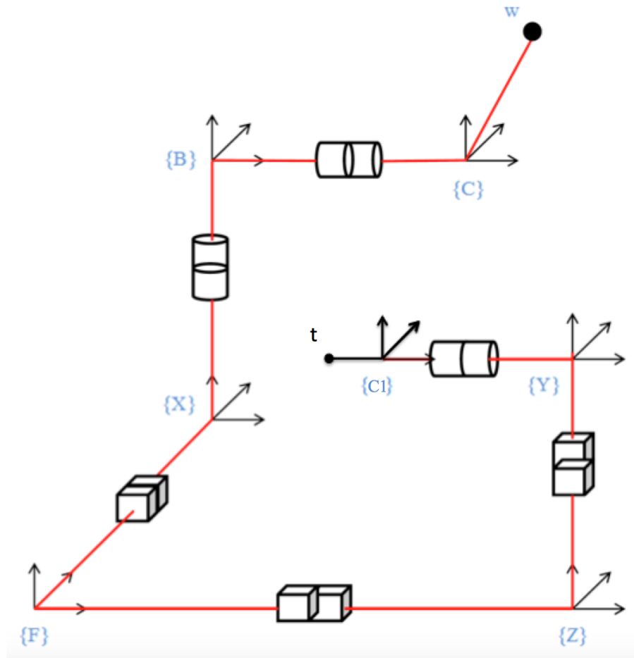
Figure 4.1 : Kinematic chain of the five-axis machine tool studied [1]
