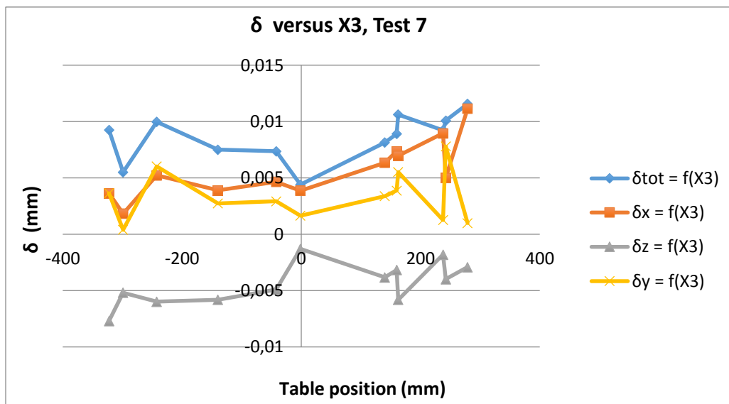
Figure 4.18 : \delta versus X3 , for test 7, influence of the table position on the rigid body motion of the table; \delta_{tot} is the total linear rigid body motion
