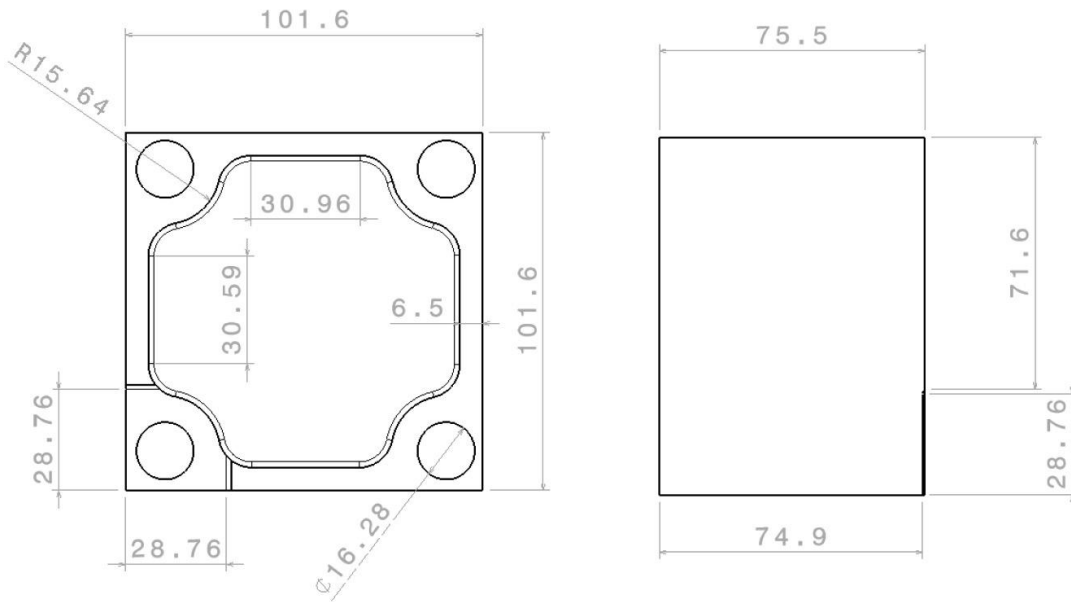
Figure 4.8 : Drawing of the spacer with nominal dimensions
