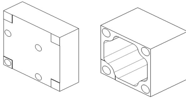
Figure 4.6 : Bloc (left) and spacer (right)
