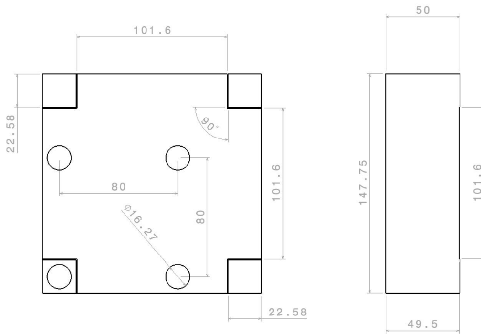
Figure 4.7 : Drawing of the bloc with nominal dimensions
