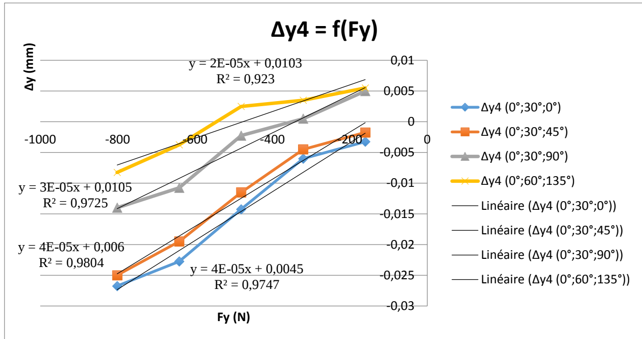
Figure 4.16 : \Delta y_4 versus F_y , with linear regression, for tests 3 to 7 and indexations (0^\circ; 30^\circ; 0^\circ) , (0^\circ; 30^\circ; 45^\circ) , (0^\circ; 30^\circ; 90^\circ) , (0^\circ; 60^\circ; 135^\circ)
