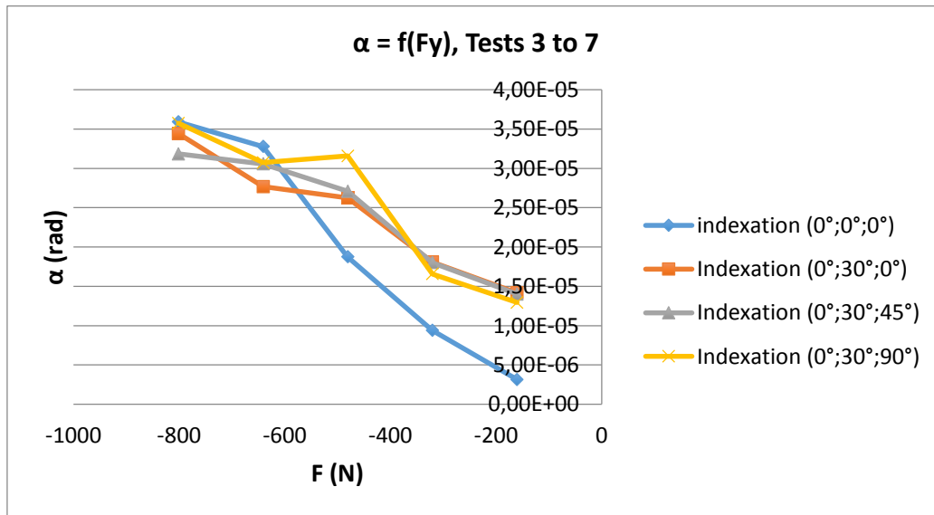
Figure 4.17 : Load effect on the rigid body motion of the table
