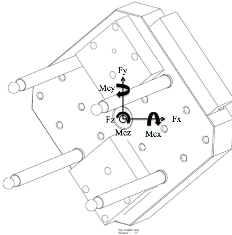
Figure 4.14 : Forces and torques in the R1 reference frame
