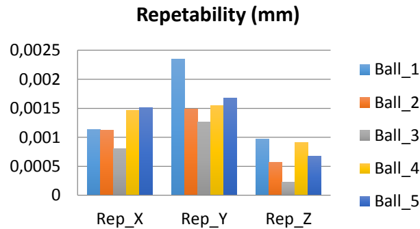
Figure 4.5 : Repeatability diagram
