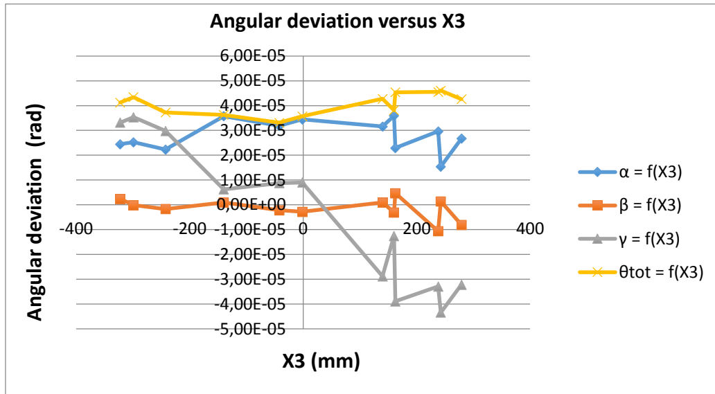
Figure 4.19 : Angular deviation versus X3, influence of the table position on the table angular deviation
