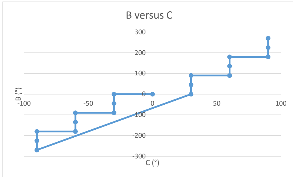
Figure 4.4 : Test Protocol – B- and C-axis indexations throughout one test
