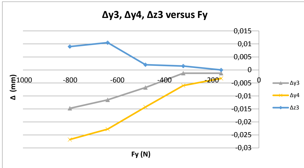
Figure 4.15 : Volumetric errors ( \Delta y_3 , \Delta y_4 , \Delta z_3 ) versus F_y , for tests 3 to 7, for B=30^\circ and C=0^\circ
