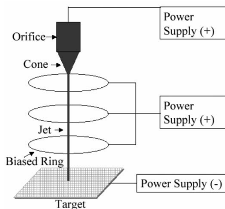
Figure 2.21: A multiple-field technique to obtain aligned fibers [167]. © 2001 Elsevier
