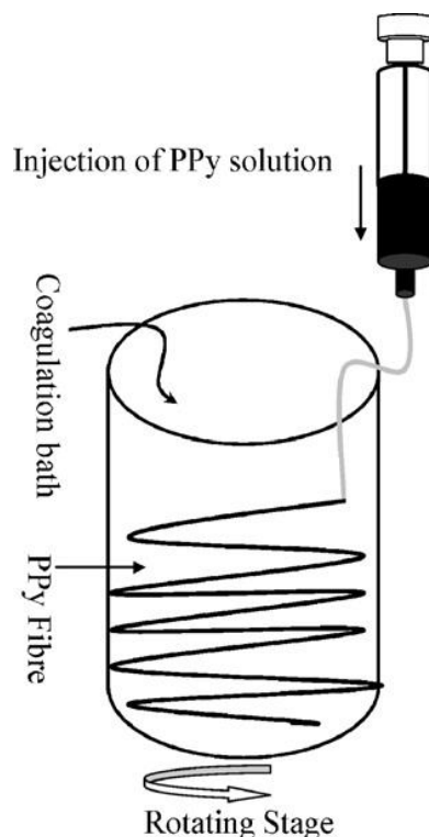
Figure 2.7: Schematic diagram of a wet-spinning apparatus [88]. © 2007 Elsevier
