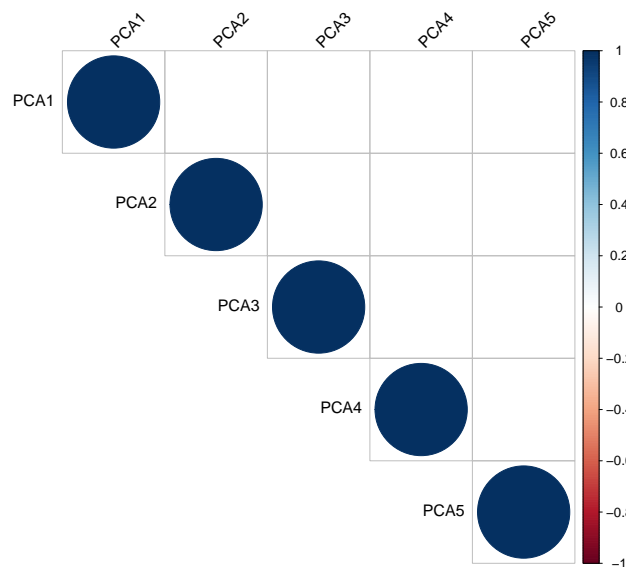
Figure 3.12 Correlation matrix after rotation
