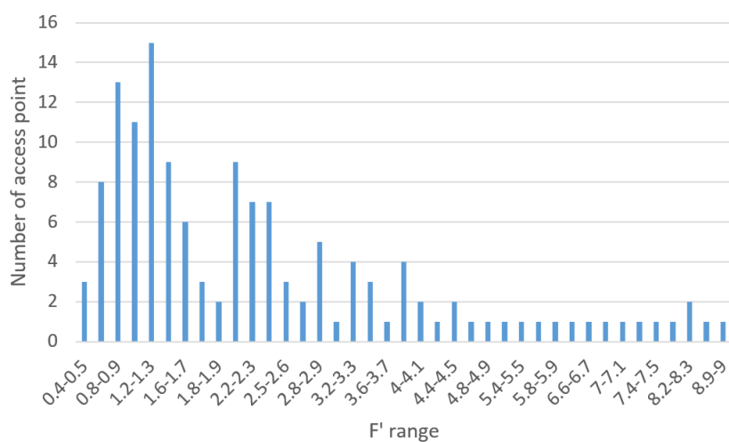
Figure 3.8 Distribution of F' range
