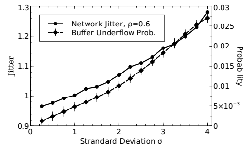
Figure 7.5 Network Jitter and Underflow Probability for Log-normal Inter-arrival Time Distribution- \rho = 0.6
