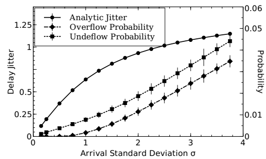
Figure 5.7 LogN/D/1/140-Large Buffer
