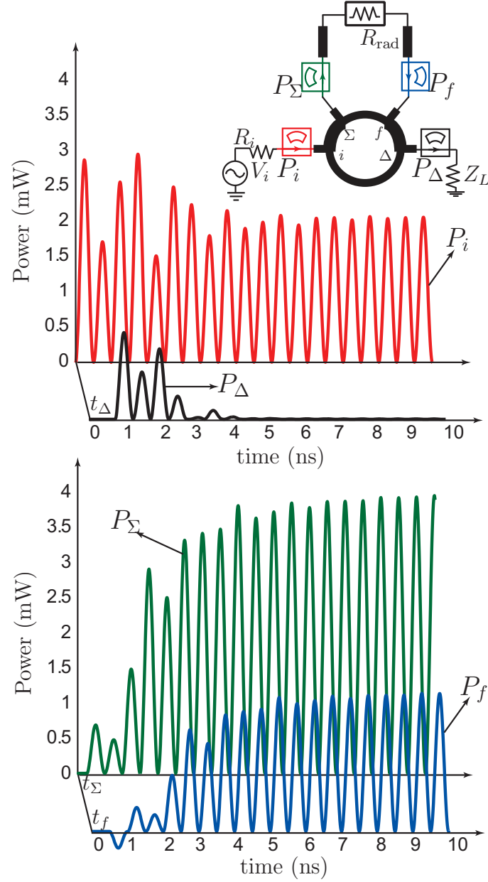
Figure 5.11 Transient response (Agilent ADS) of the 3-dB power-recycling LWA system of Fig. 5.8, using an ideal rat-race coupler, ideal feeding TLs of length \ell_{45} = \ell_{63} = 3\pi/4 , and a 3-dB resistive attenuator. The system is excited by a 1 GHz harmonic source of peak voltage V_i = 0.316 V (0 dBm in a 50 \Omega system).
