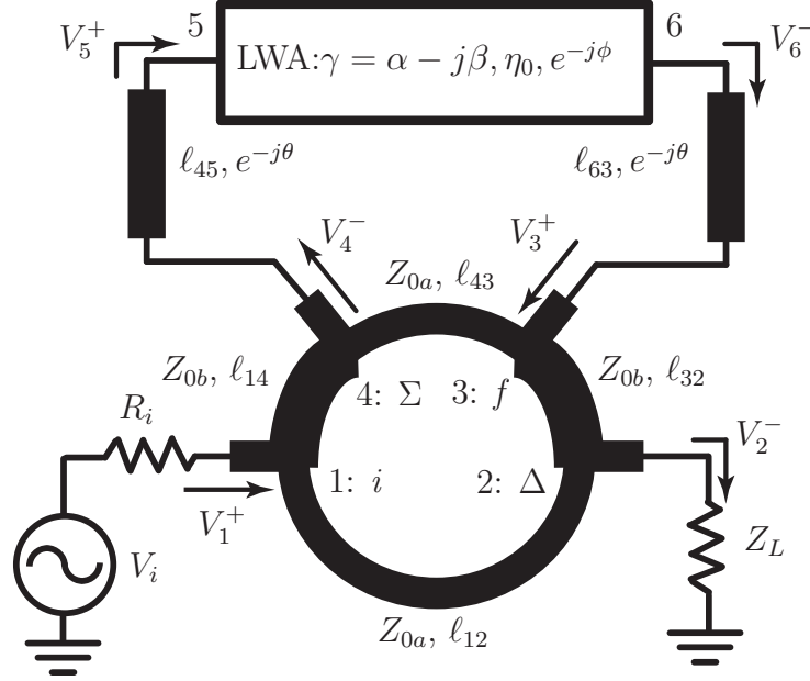
Figure 5.8 Rat-race based implementation of the power-recycling LWA system shown in Fig. 5.7. In general, the rat-race exhibits different power combining ratios, corresponding to two sets of impedances ( Z_{0a} and Z_{0b} ), depending on the open loop-efficiency \eta_0 of the LWA. Notation for the 180^\circ hybrid ports: i : input, f : feedback, \Sigma : sum, and \Delta : difference.
