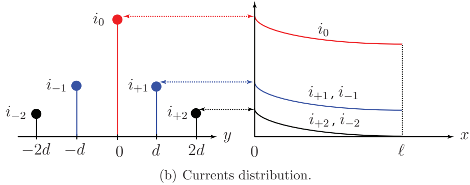
Figure 5.1 Proposed CRLH TL LWA array with improved efficiency using a series feeding network for power recycling. (a) Perspective view. (b) Current distribution in x - and y -directions.
