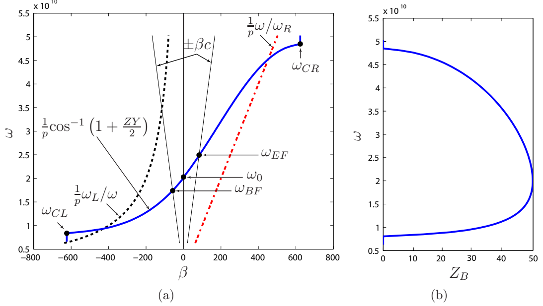
Figure 1.2 a) Dispersion diagram ( \beta - \omega diagram), and b) Z_B of a CRLH TL for the following unit cell parameters: L_R = L_L = 2.5 nH and C_R = C_L = 1.0 pF.
