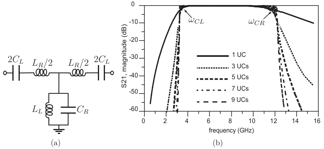
Figure 3.1 Conventional CRLH structure. (a) UC equivalent circuit model. (b) Transmission response as a function of the number of UCs.
