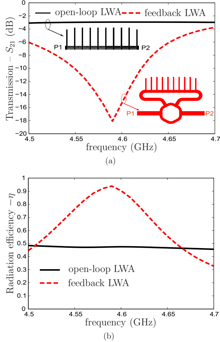
Figure 5.10 Full-wave (MoM, Ansoft Designer) demonstration of a 3-dB power-recycling LWA system designed at 4.58 GHz in the lossless case (neither ohmic nor dielectric losses), comparing the open loop LWA (Fig. 5.6) and the power-recycling LWA (Fig. 5.8). The LWA is an interdigital/stub CRLH LWA [4] with the parameters: number of unit cells: N = 10 , unit cell length: p = 208 mils, number of fingers: N_f = 6 (3 pairs), finger width: w = 15 mils, inter-finger gap: g = 6 mils (everywhere), stub width: w_{stub,1} = 39 mils, length of first and last stubs: L_{stub,2} = 580 mils, length of other stubs: L_{stub} = 644 mils, substrate thickness: h = 62 mils, substrate permittivity: \epsilon_r = 2.2 . a) S-parameters. b) Radiation efficiency.
