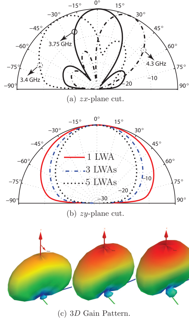
Figure 5.2 Simulated radiation patterns using Ansoft Designer software. (a) zx -plane cut of normalized gain radiation patterns at the three frequencies 3.4 GHz, 3.75 GHz and 4.3 GHz illustrating beam-scanning from backward through broadside to forward directions of the CRLH TL LWA with N = 1 element. (b) zy -plane cut of normalized gain radiation patterns at broadside frequency of 3.75 GHz for an array of N = 1, 3 and 5 TL LWA elements. (c) 3D plot of gain radiation pattern for an array of N = 1, 3 and 5 TL LWA elements (from left to right).
