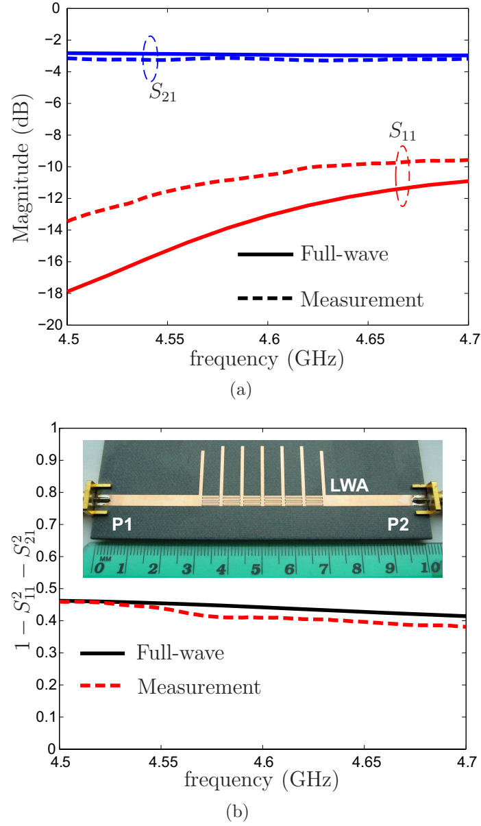
Figure 5.13 Full-wave simulated (MoM, Ansoft Designer) and measured scattering parameters for the 3-dB CRLH LWA prototype shown in the inset, which has the parameters given in Fig. 5.10, except for the number of unit cells which is here N = 7 . (a) Return and insertion losses. (b) Dissipated power ratio, including radiation and loss power.
