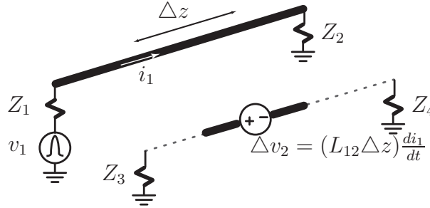
Figure C.4 An equivalent model of magnetic coupling in coupled-line couplers as an emf voltage source in series with TL 2.
