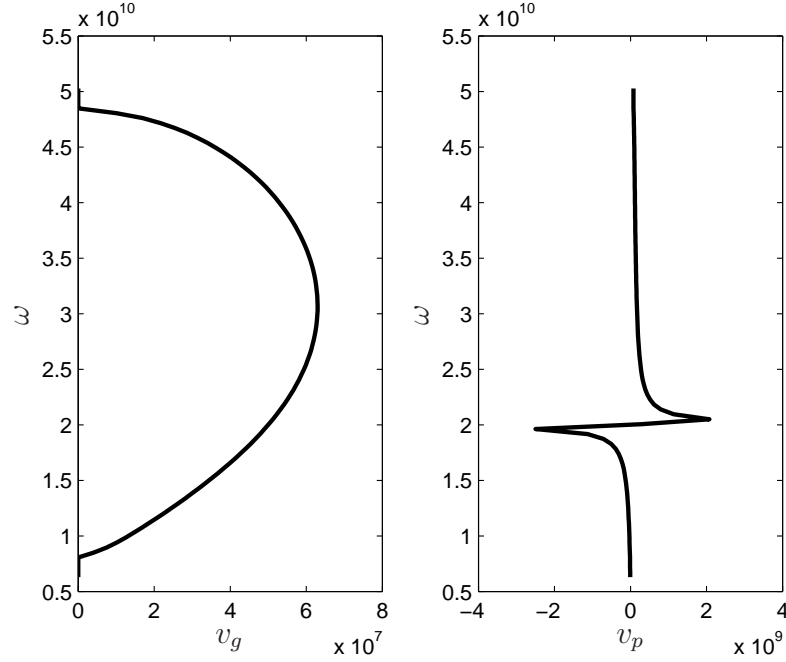
Figure 1.3 Group and phase velocities of a signal propagating along the CRLH TL structure with the same UC parameters given in the caption of Fig. 1.2.1.
