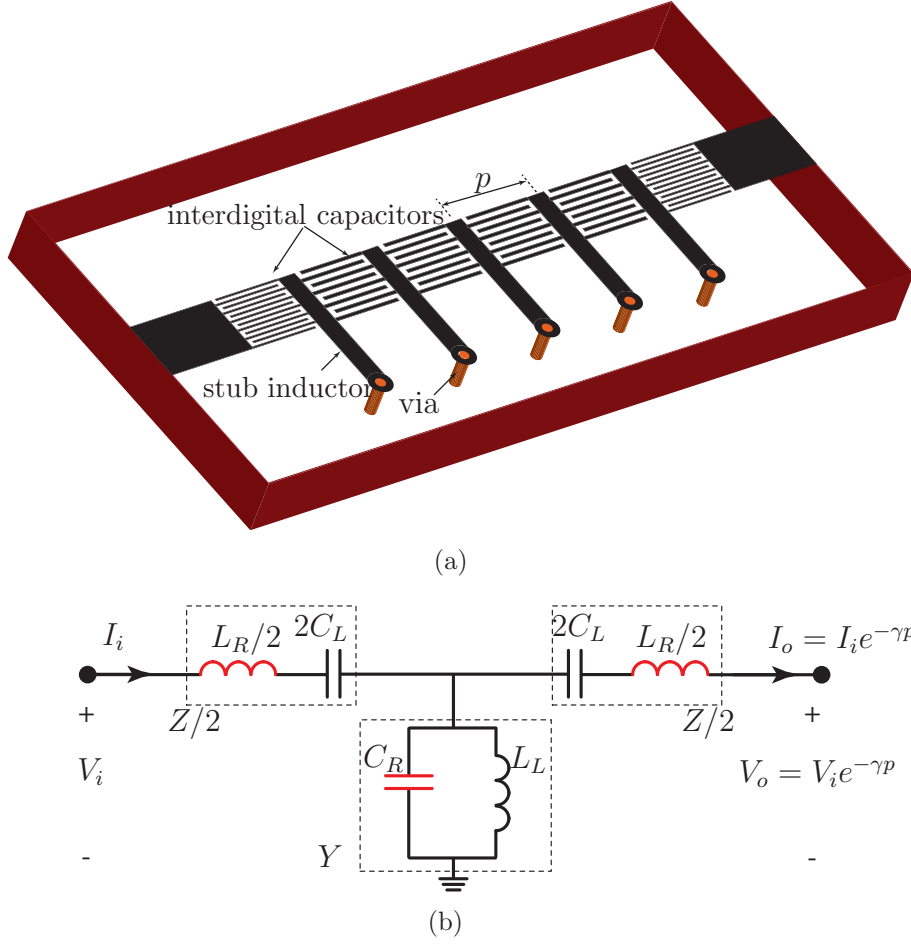
Figure 1.1 a) Planar CRLH TL MTM with interdigital capacitor and shorted stub inductor. b) Equivalent LC circuit model of a UC.
