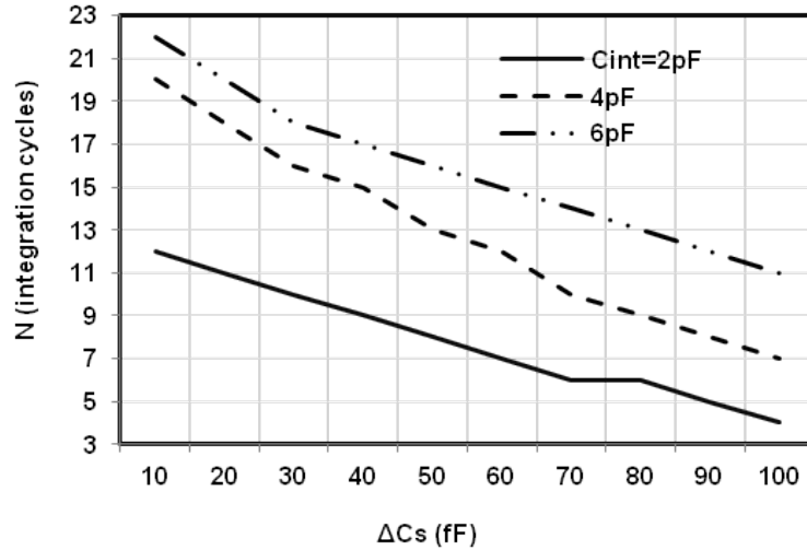
Figure 5.14: The maximum number of N for different integrating capacitance ( C_{int} ) value.
