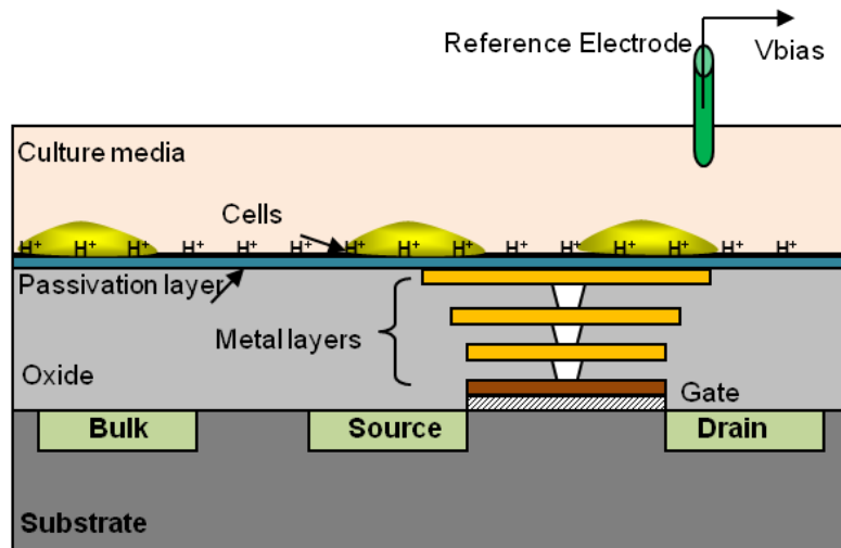
Figure 2.5: Schematic diagram of ISFET pH-sensor, the gate is connected to the pH-sensitive membrane by stacking metal layers.
