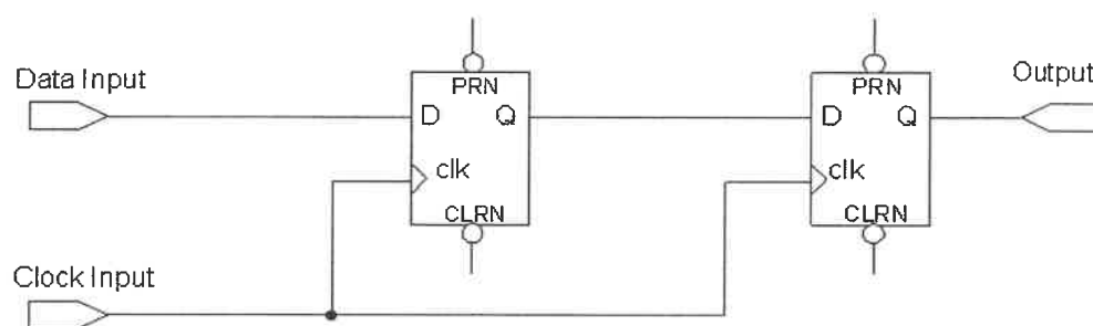
Figure 2. 6 Multiple-stage synchronizer
