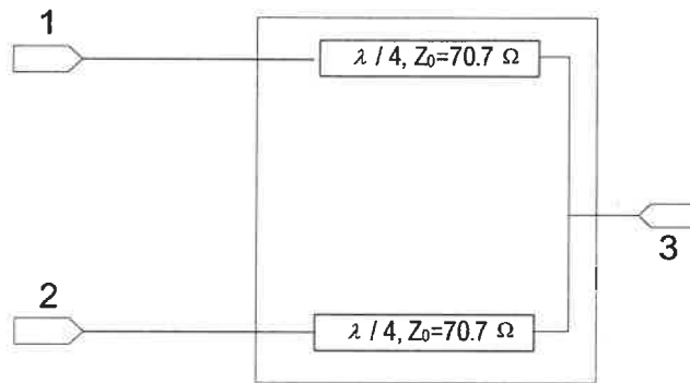
Figure 3.2 Model 2: unisolated combiner
