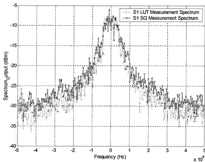
Figure 2.23 S 1 spectrum between LUT and SRFB from measurement
