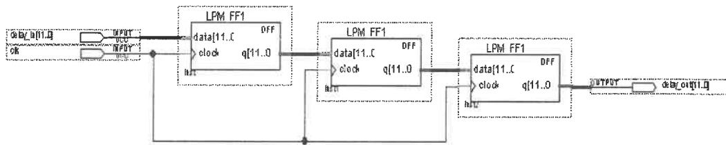
Figure 2.9 Three LPM_FF block for a three clock cycle delay
