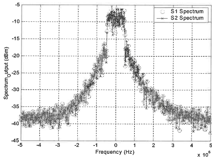
(a) Constant envelope phase modulated signals S_1 and S_2
