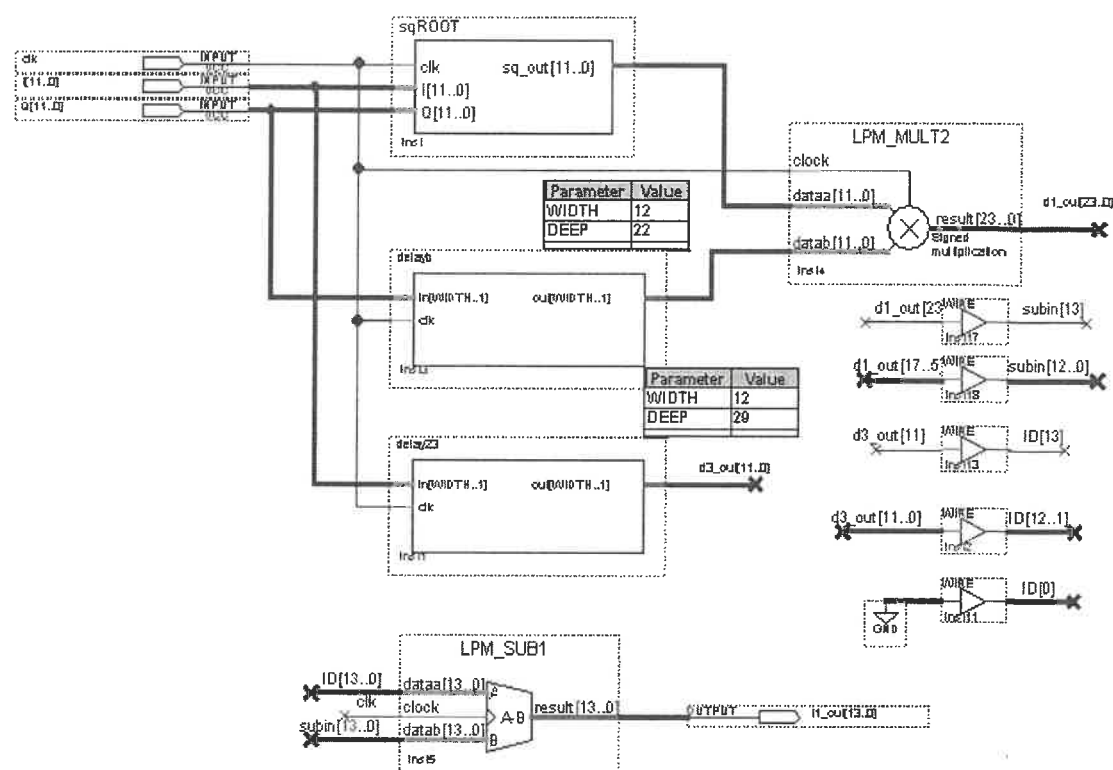
Figure 2.13 Top level design for I_1(n) with SRFB in the Quartus II 2.0
