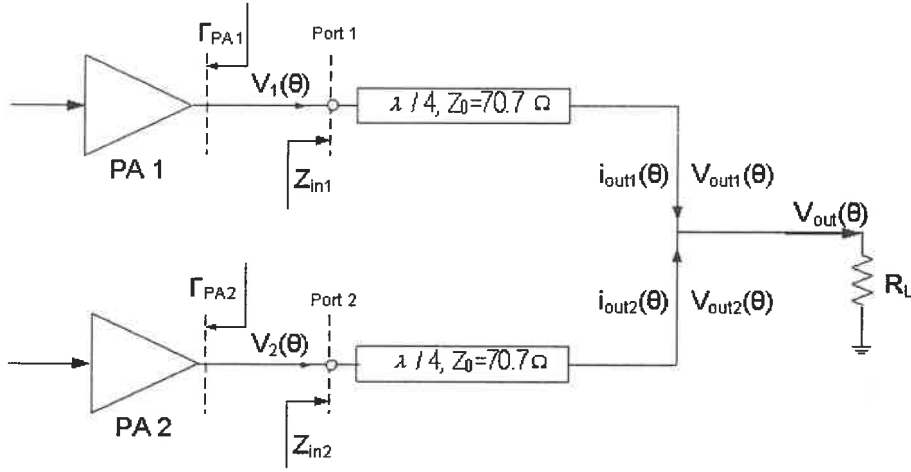
Figure 3.5 Lossless combiner analysis
