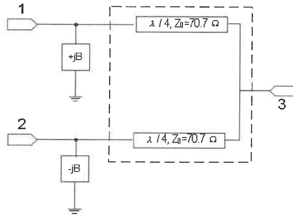
Figure 3. 6 Chireix outphasing system with shunt susceptances
