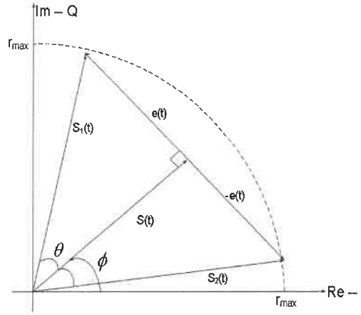
Figure 2. 2 Decomposition of signals in the signal component separator
