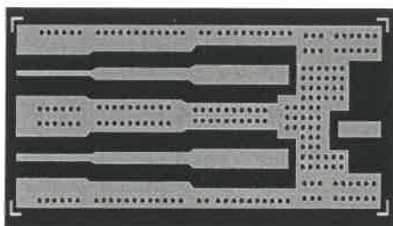
(a) Layout diagram
