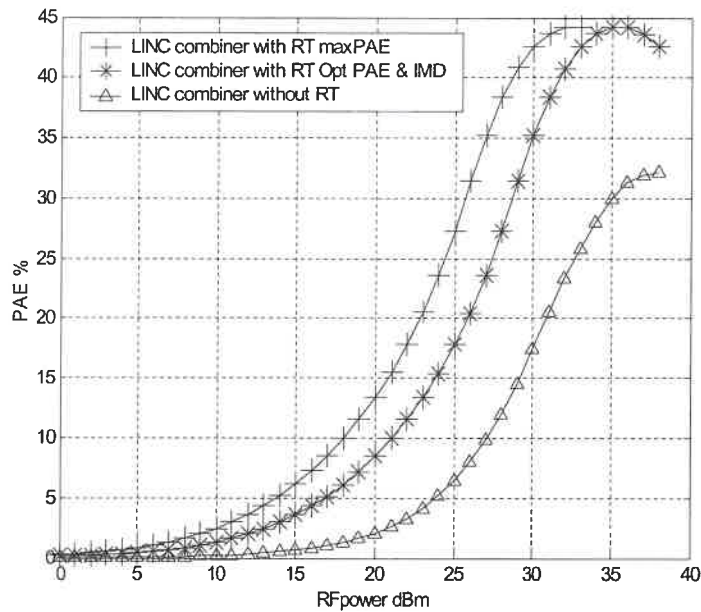
Figure 3.12 PAE \eta (%) vs Pin (dBm) with two-tone signal
