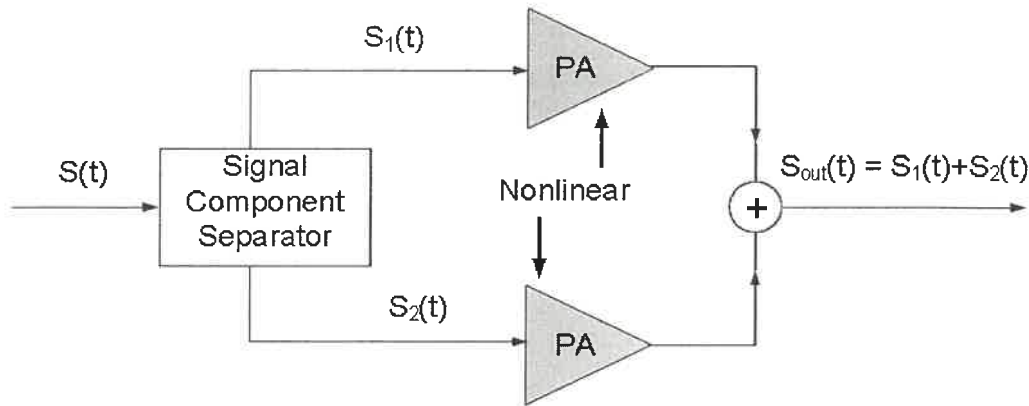
Figure 2. 1 Basic schematic diagram of the LINC transmitter
