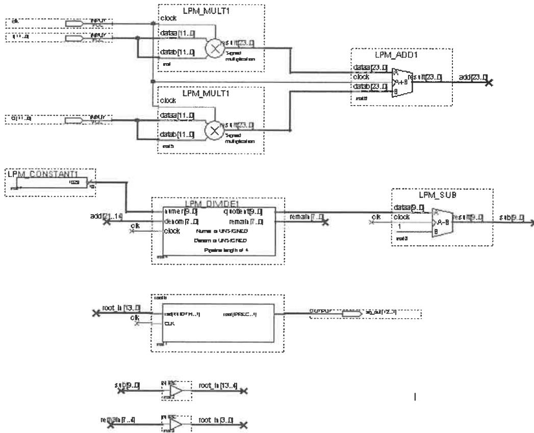
Figure 2.12 SR_Part implementation of SRFB in the Quartus II 2.0
