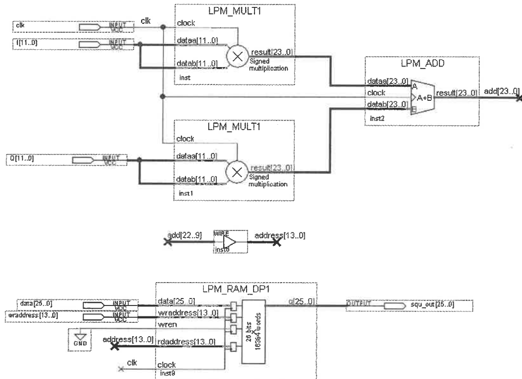
Figure 2.8 LUT 16384 design block in Quartus II 2.0
