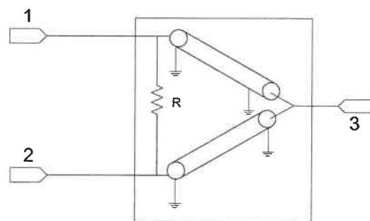
(b) Wilkinson combiner
