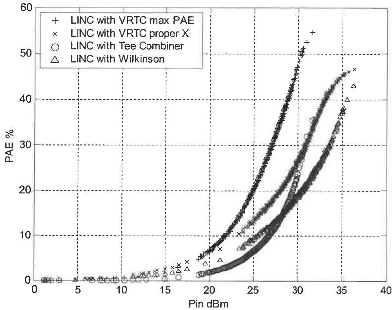
Figure 3.13 PAE curves with IS95 signal
