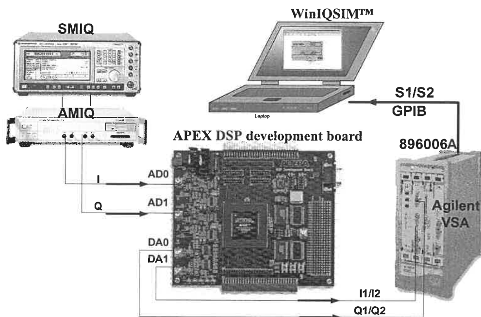
Figure 2. 21 Measurement set-up
