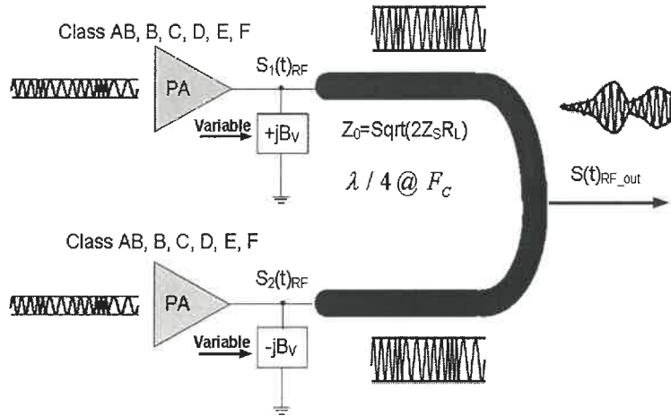
Figure 1.5 Variable reactive termination combiner
