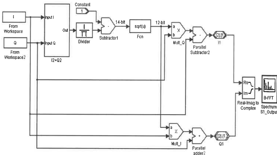
Figure 2. 15 Top level design for S_1 in Simulink ---- method 2 SRFB
