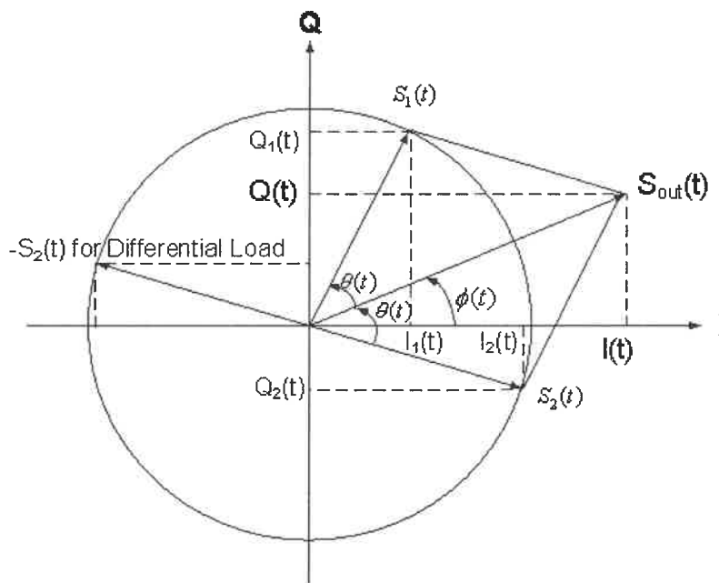
Figure 2.3 Vector diagram illustrating relationship between components
