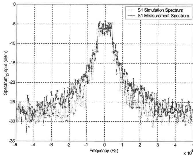
Figure 2.24 Spectrum comparison between simulation and measurement
