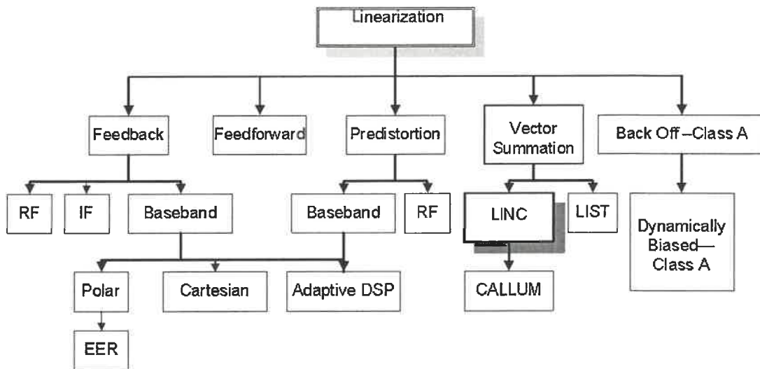
Figure 1.1 RF amplifier linearization techniques
