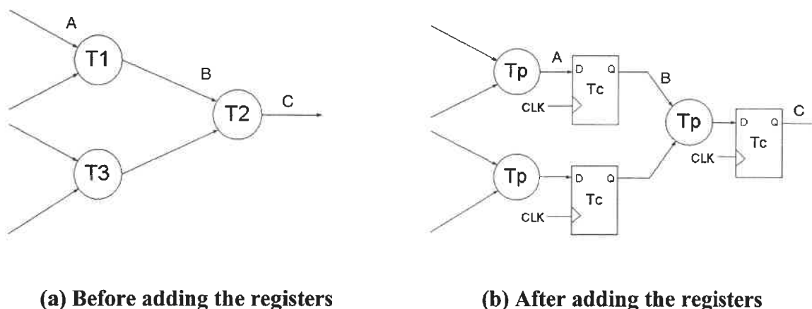
Figure 2.5 A combinatorial design and a pipeline design
