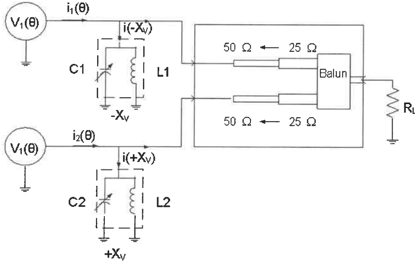
Figure 3. 9 Implementation of variable reactive termination combiner
