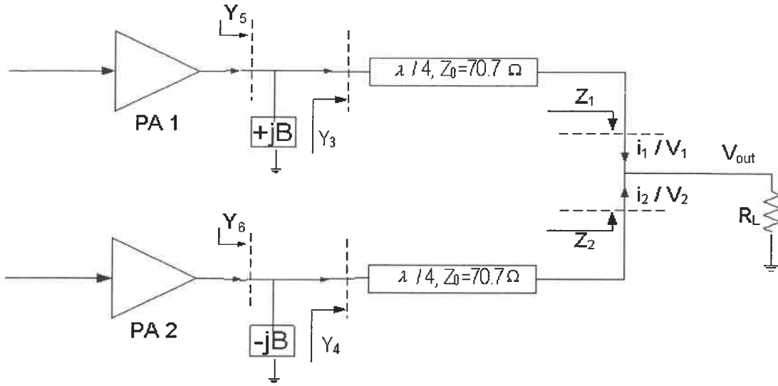
Figure 3. 7 Chireix outphasing system analysis
