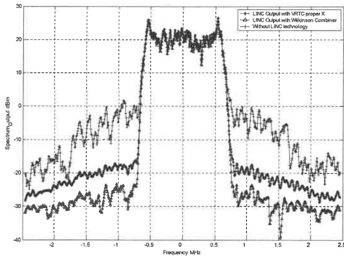
Figure 3.14 LINC output spectrum using an IS95 REV signal
