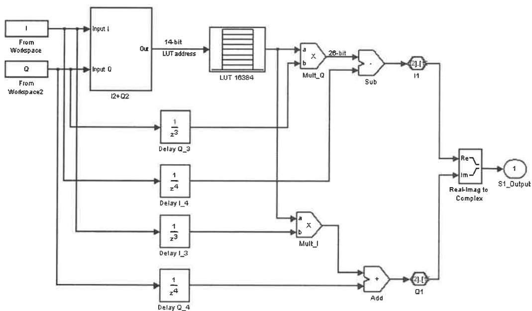
Figure 2.14 Top level design for S_1 in Simulink ---- method 1 LUT
