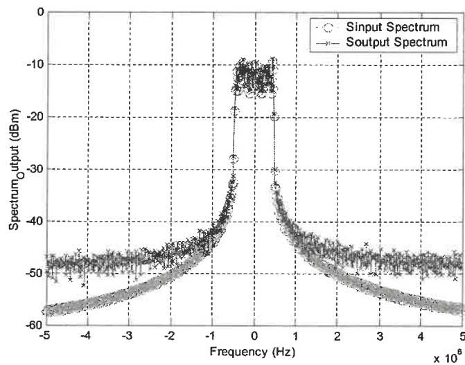
(b) LINC output S_{\text{output}} and input signal S_{\text{input}}
