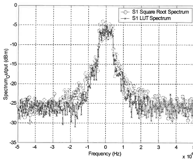
Figure 2. 20 S 1 spectrum comparison between LUT and SRFB
