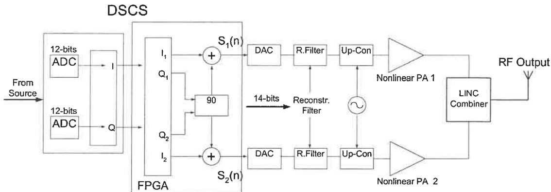
Figure 2. 4 LINC implementation with a new DSCS architecture
