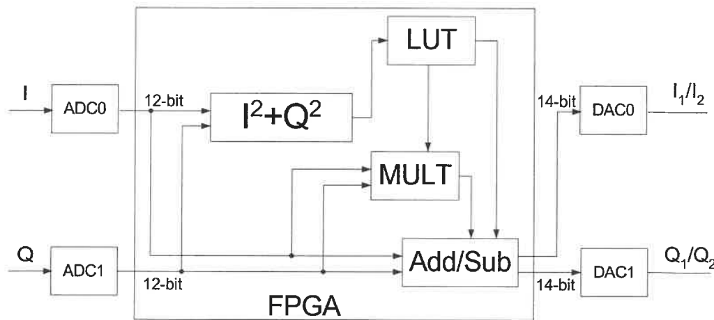
Figure 2. 7 Method 1 ---LUT design block diagram
