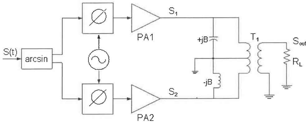
Figure 1.2 Analog LINC transmitter
