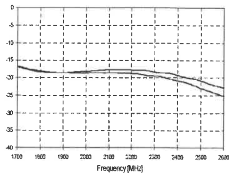
(b) 3W525 return loss
