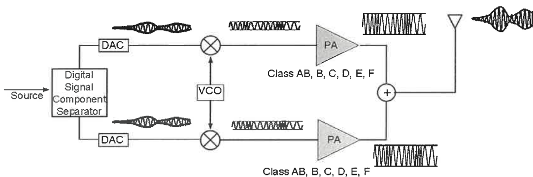
Figure 1.4 LINC transmitter using DSP technique
