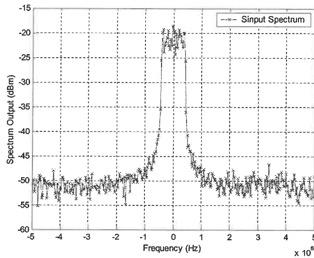
(a) Input IS95 signal in frequency domain
