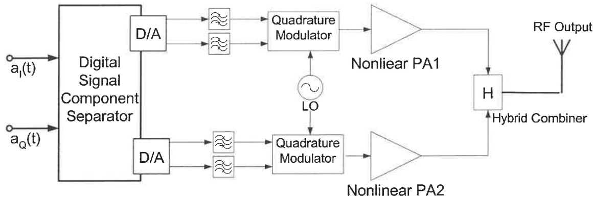
Figure 1.3 LINC transmitter with digital signal component separator
