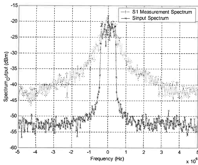
(a) S_1 and S_{\text{input}} from measurement
