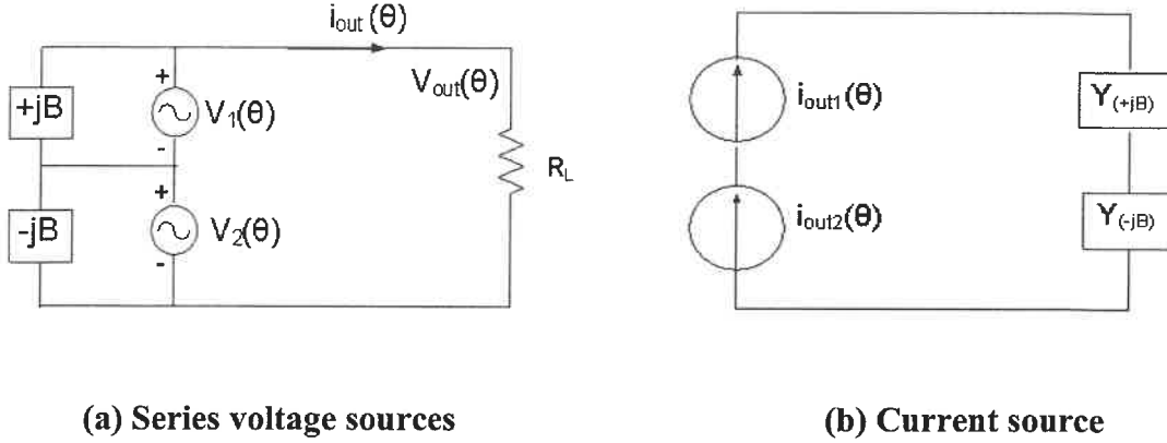
Figure 3.4 Voltage and current models with shunt susceptances
