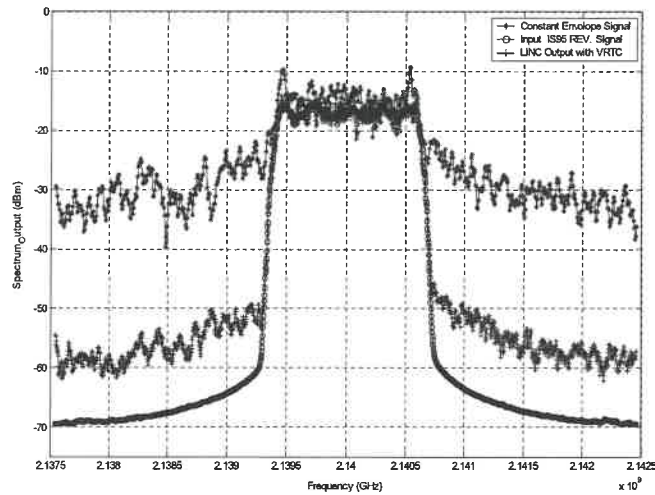
(a) IS95-Reverse link CDMA signal
