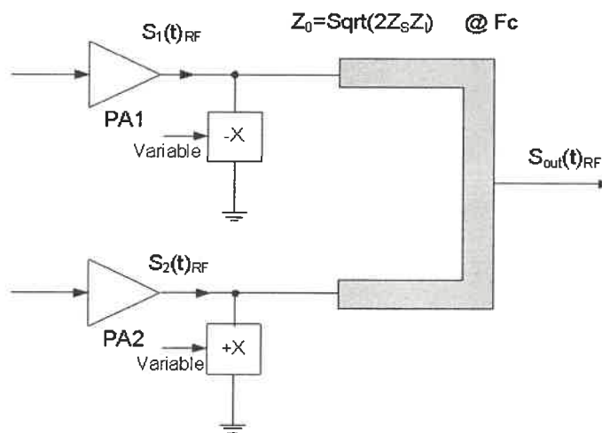
Figure 3. 8 Variable reactive termination combiner
