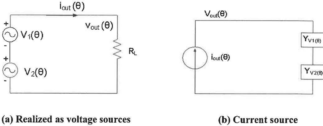
Figure 3.3 LINC combiner realized voltage / current sources
