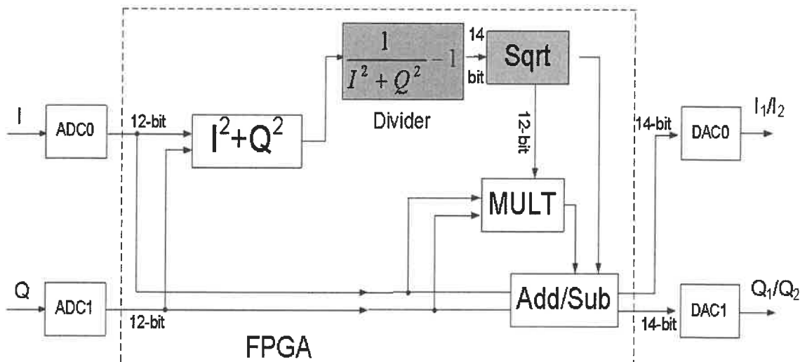
Figure 2. 11 Method 2 - Square-Root Function Block design diagram
