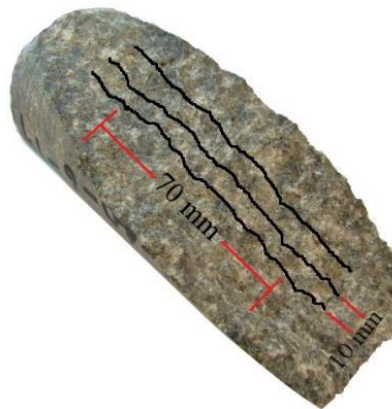
Figure 3-7: Roughness profiles selected in the middle part of the fracture surface.
