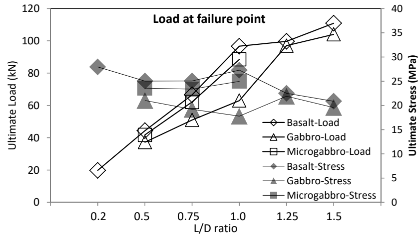
Figure 4-7: Variation of average ultimate loads and stresses at failure point with L/D ratio in three rock types.
