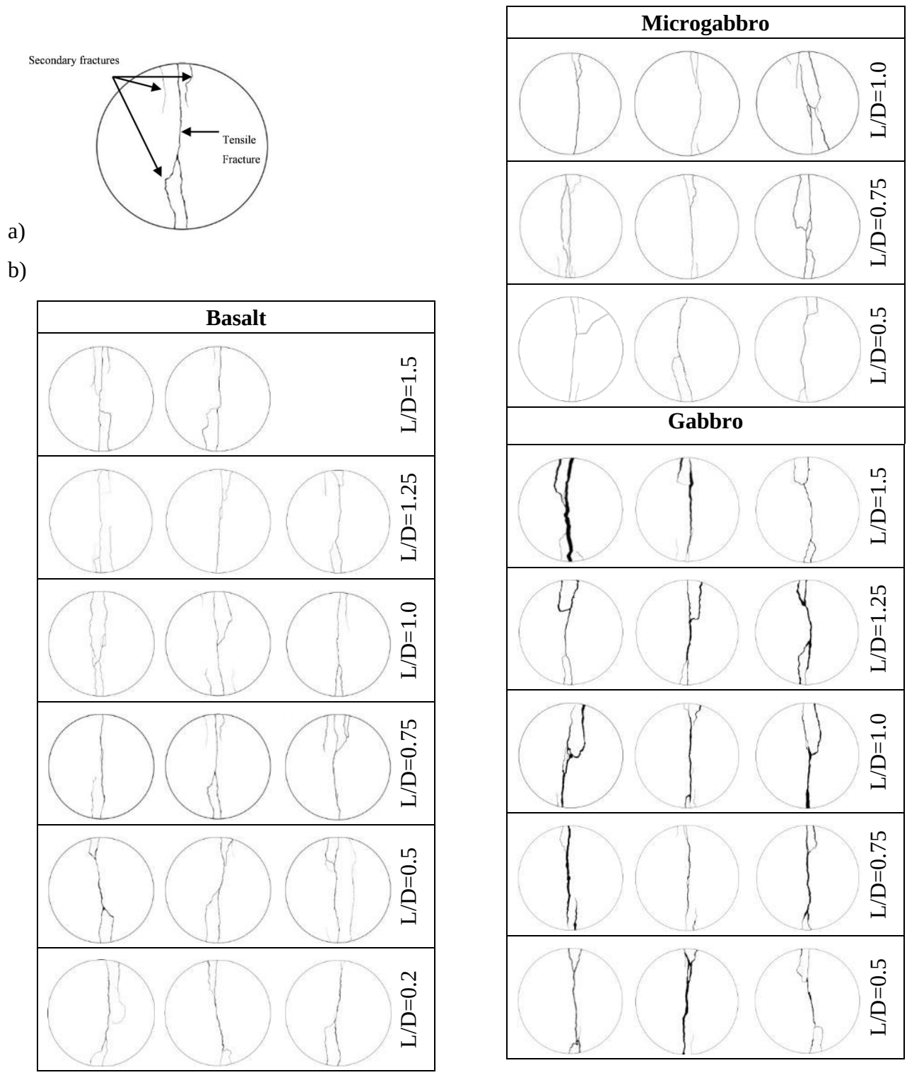
Figure 4-10: a) Fracture types observed in the split samples; b) Fracture pattern of the three rock types with different L/D ratios.
