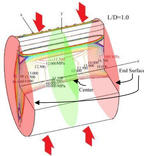
Figure 4-18: Tensile stress distribution in the specimen with L/D=1.0 obtained by 3D FEM analysis (adapted from Yu et al., 2006).
