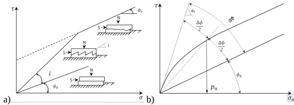
Figure 2-13: a) Patton's shear strength bi-linear criterion (1966). b) Non-linear criterion developed by Maksimovic (1996).
