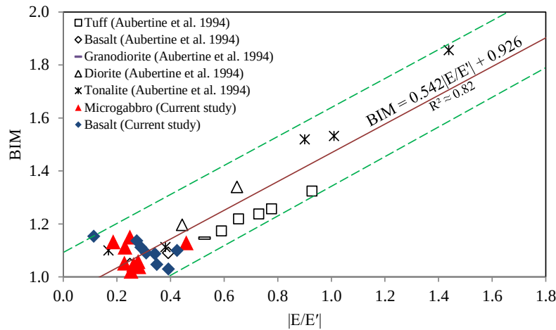
Figure 5-11: Empirical correlation between BIM and |E/E'| for fine-grained rocks.
