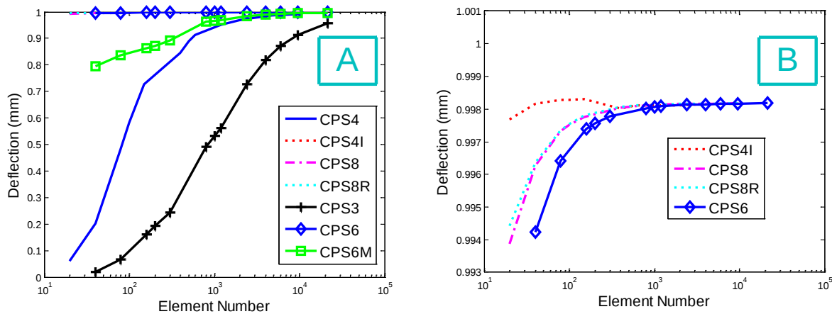
Figure 6-3 : Cantilever beam end deflection, (B) is the zoom of the superimposed lines in the figure (A)
