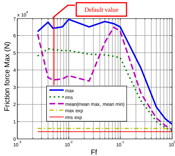
Figure D–7 : Slip tolerance (fraction F_f ) effect on the friction force (decay)
