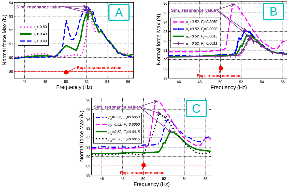
Figure 6-18 : Contact normal force, (A) Lagrange formulation, penalty formulation: (B) F_f sensitivity and (C) \mu_c sensitivity
