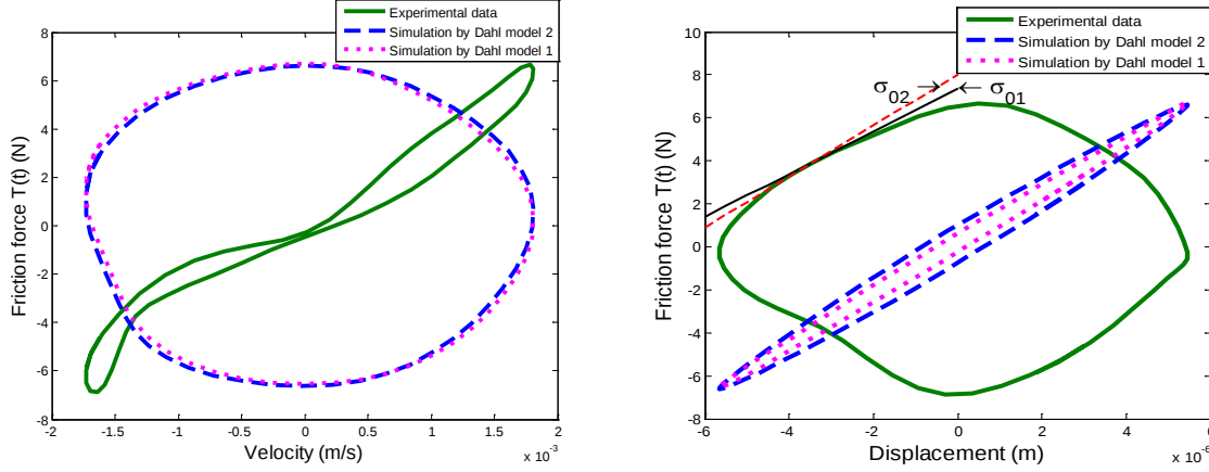
Figure B-13 : Friction force and Dahl model
