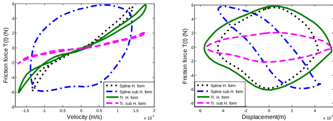
Figure C–6 : Friction force
