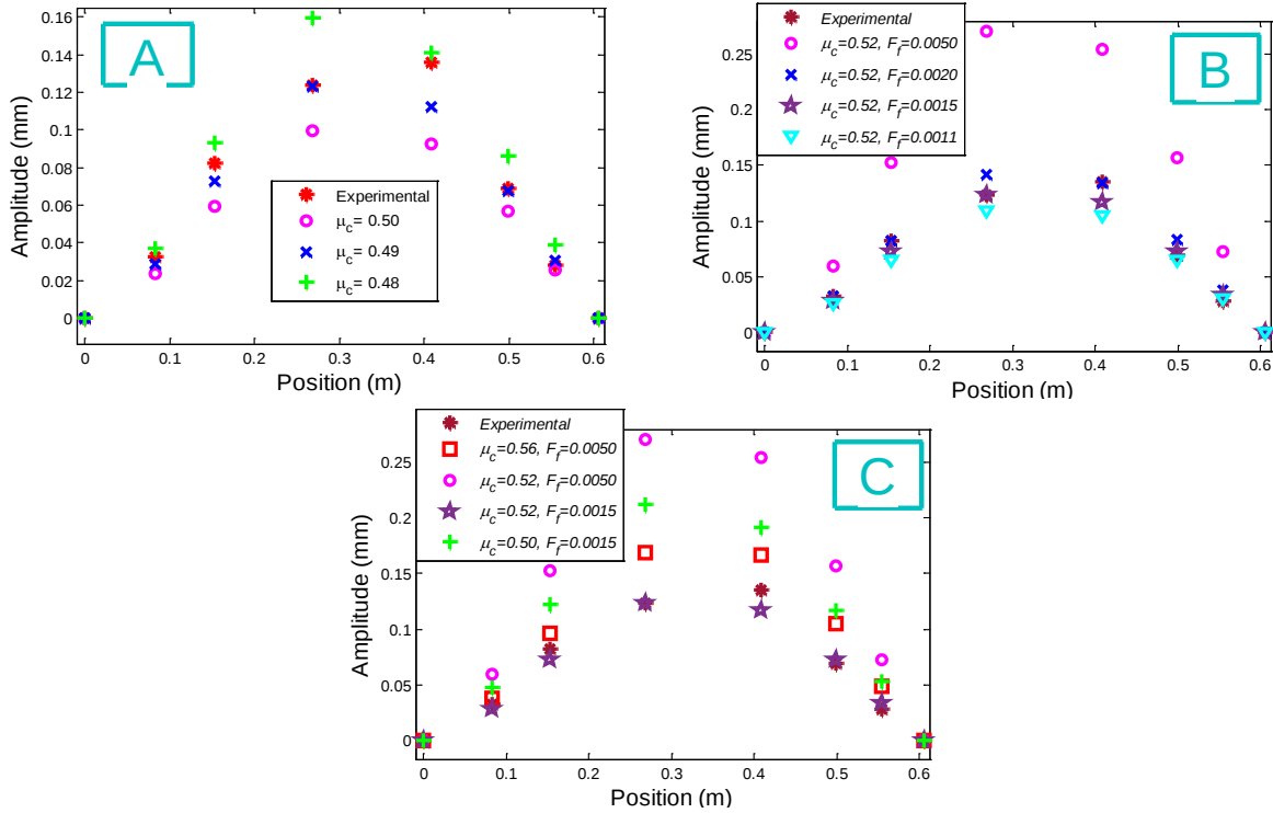
Figure 6-13 : Beam response envelope (deflection maximal), (A) Lagrange formulation, penalty formulation: (B) F_f sensitivity and (C) \mu_c sensitivity)
