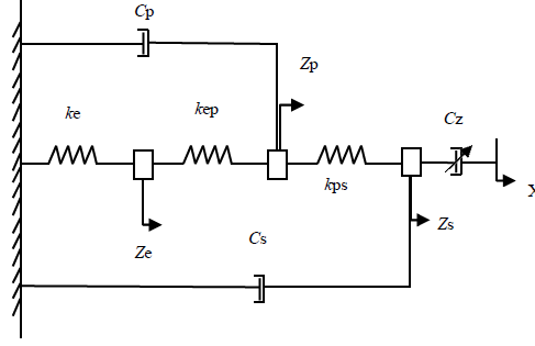
Figure 5-17 : Schematic of the hybrid friction model (Azizian, 2012)
