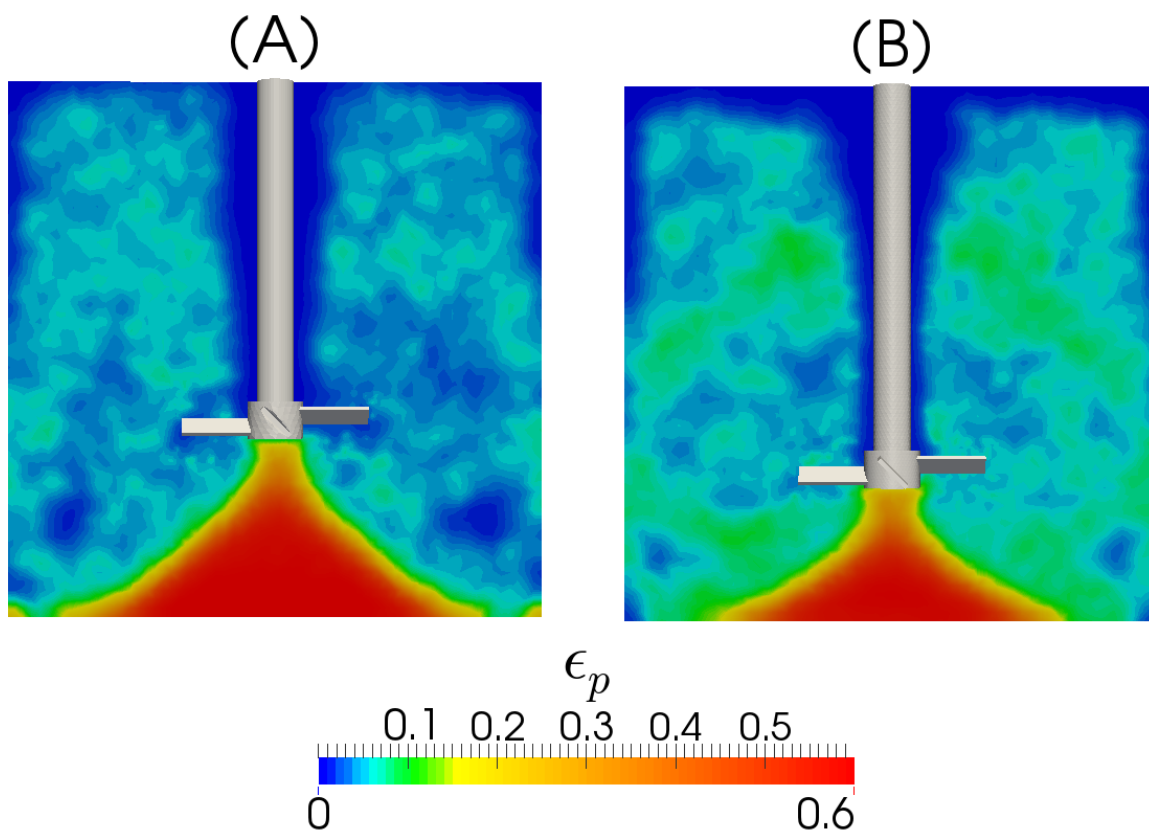
Figure 10.18 Solid volume fraction ( \epsilon_p = 1 - \epsilon_f ) on the P_y cross-section at N = 650 RPM for (A) C = T/3 and (B) C = T/4
