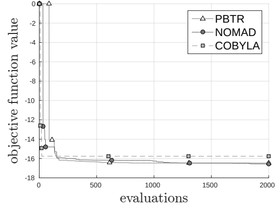
(b) SIMPLIFIED_WING.
