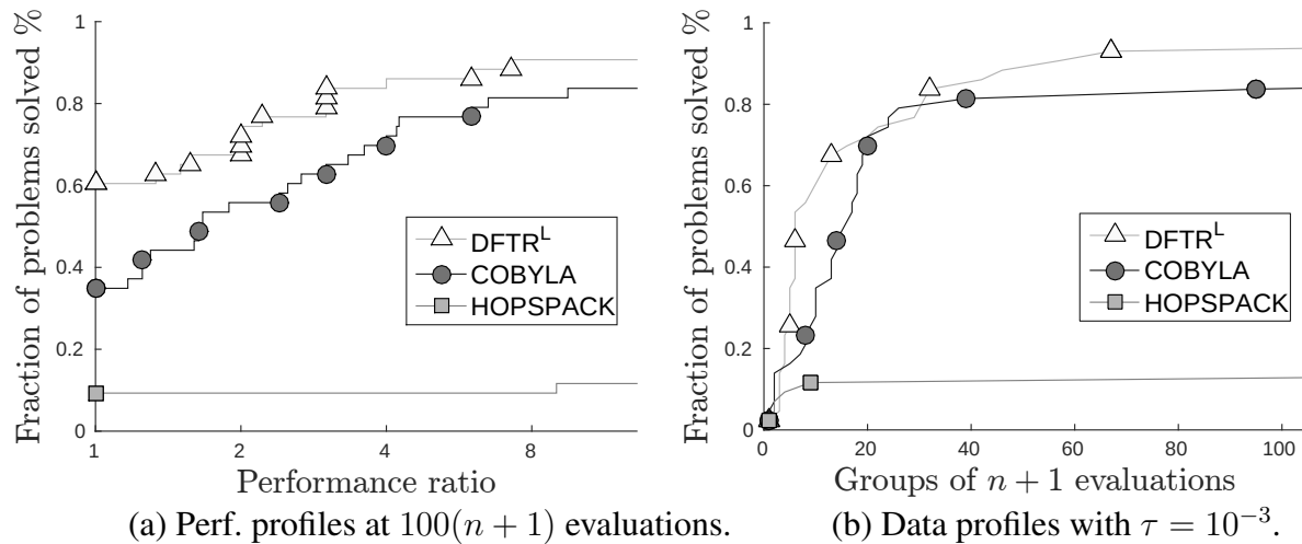
Figure 6.2 Comparison of DFTR L with COBYLA and HOPSPACK on analytical CUTEst problems with at least one equality.
