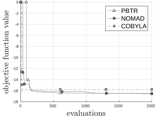
(a) AIRCRAFT_RANGE.
