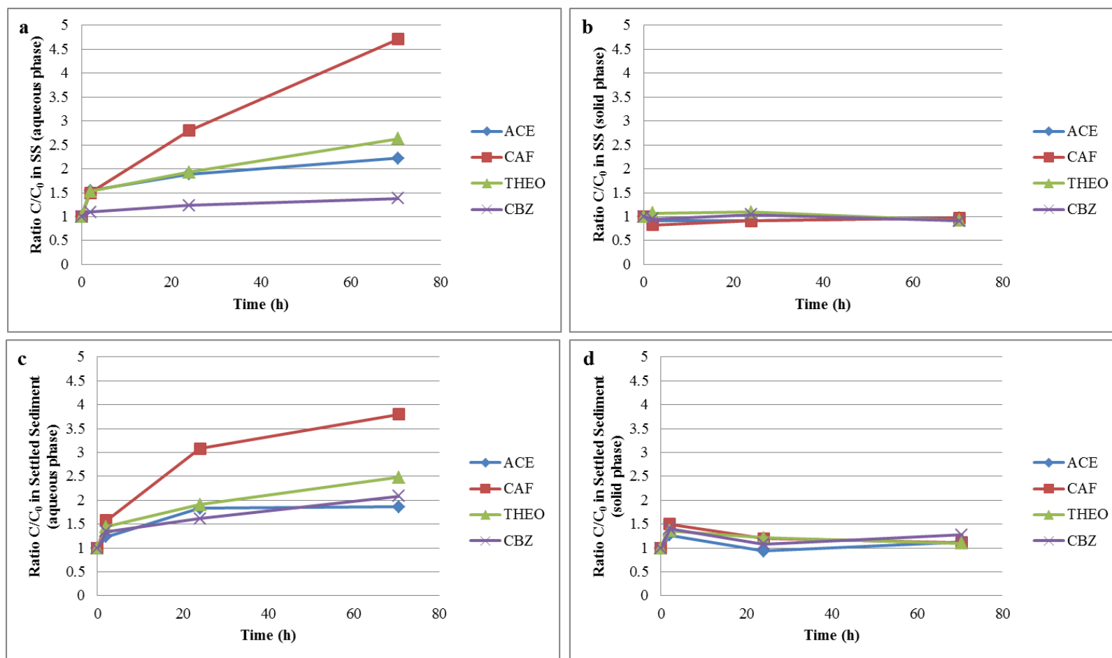
Figure 5.3. Desorption as a function of time without spiking and with shaking (Reactors C) expressed in C/C_0 ratio of the selected pharmaceuticals except CBZ-DiOH in aqueous phase of SS (a) and StS (c) and in solid phase of SS (b) and StS (d) C and C_0 correspond to the concentrations in aqueous phase ( \text{ng L}^{-1} ) or in solid phase ( \text{ng g}^{-1} ) at defined time and 0h of desorption respectively.
