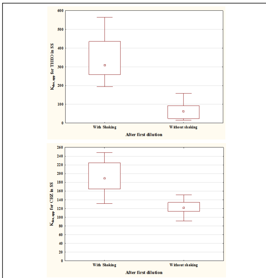
Figure 5.14. Box plots to compare distributions of pharmaceuticals after the first dilution with shaking (2x
