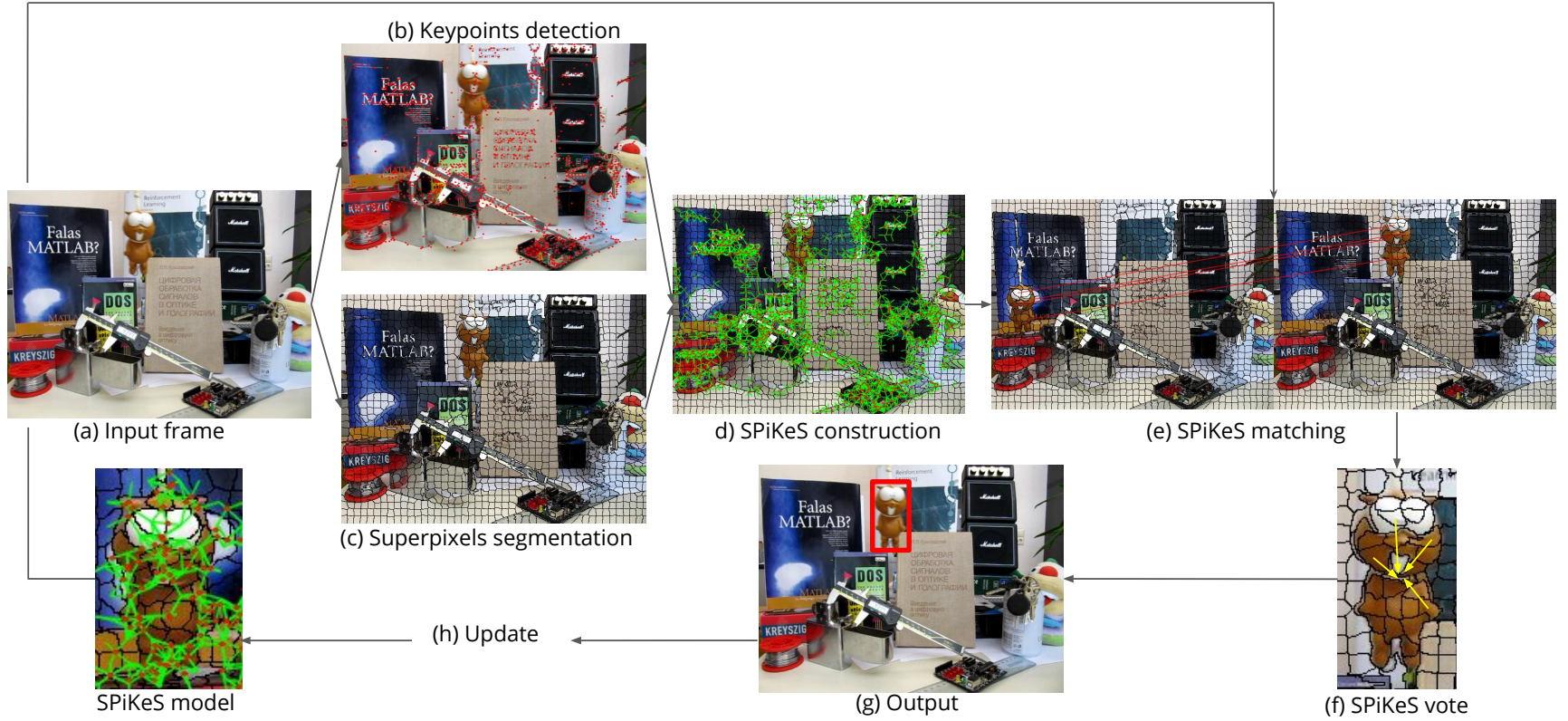
Figure 4.3 Tracking steps of our SPiKeS-based tracker. Keypoints detection (b) and superpixels segmentation (c) are processed on an input frame (a). Each superpixel forms a SPiKeS with its surrounding keypoints (d). Our SPiKeS model is matched with the new SPiKeS and the matching ones vote for the target's center (f). The model is updated from the estimated bounding box (g) if no occlusion occurs.
