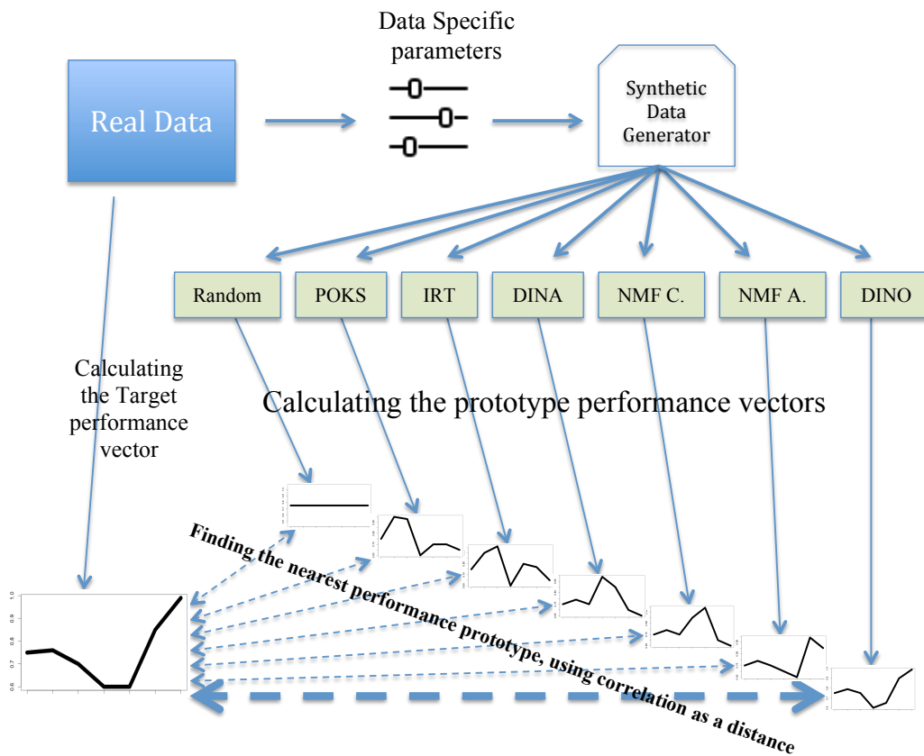
Figure 3.1 Signature framework
