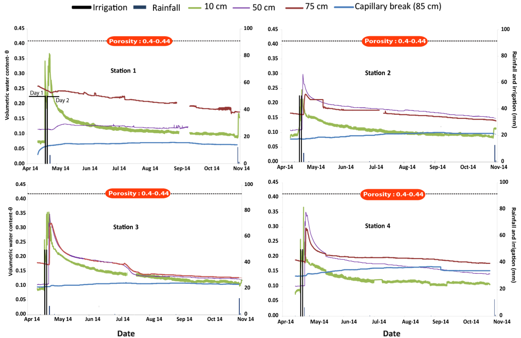
Figure 4.6 : Time trends for volumetric water content at depths of 10, 50, 75 and 85 cm for the 4 stations in the inclined experimental SR cover from April 2014 to November 2014
