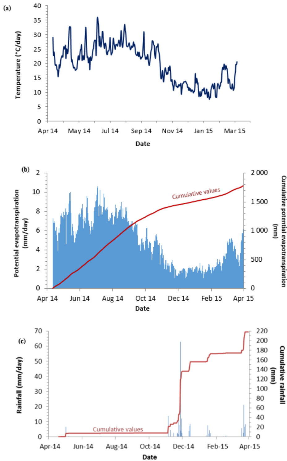
Figure 4.5 : Average daily air temperatures (a), potential evapotranspiration (b), and rainfall (c) from April 2014 to April 2015 in the study area
