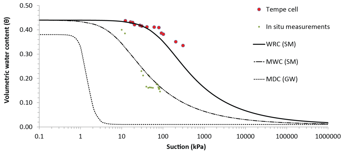
Figure 4.4: Measured and fitted water retention curves (WRCs) of fine- and coarse-grained material placed in the experimental cell; MDC is the main drying curve and MWC is the main wetting curve
