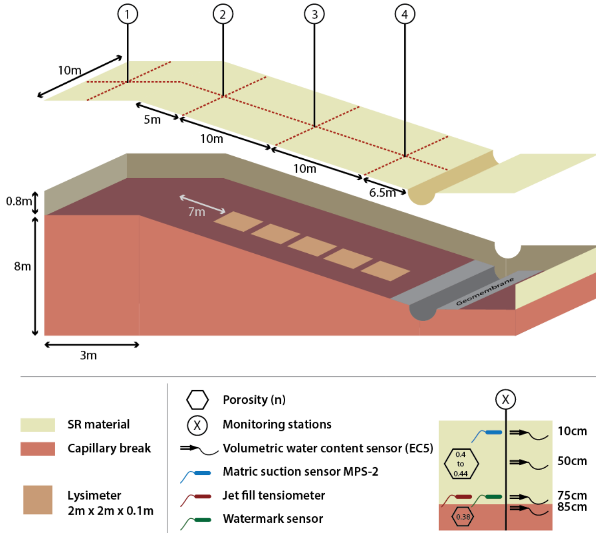
Figure 4.1 : 3D schematic representation of the inclined SR field experimental cell and corresponding instrumentation sensors
