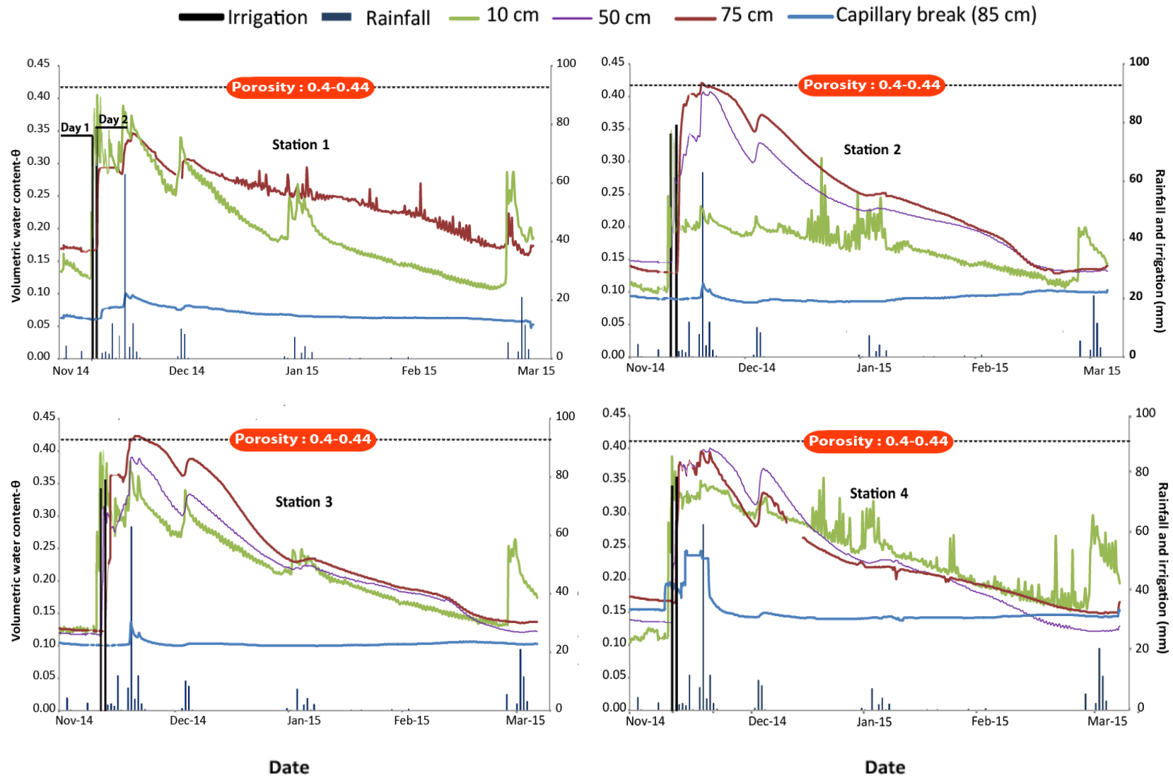
Figure 4.8 : Time trends for volumetric water content at depths of 10 cm, 50 cm, 75 cm and 85 cm for the inclined experimental SR during the second artificial rainfall event reinforced by another natural rainfall event, from November 2014 to the end of March 2015
