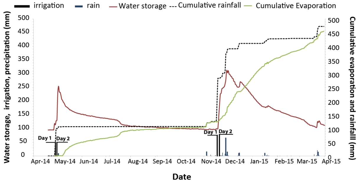
Figure 4.10 : Daily water balance for Station 3
