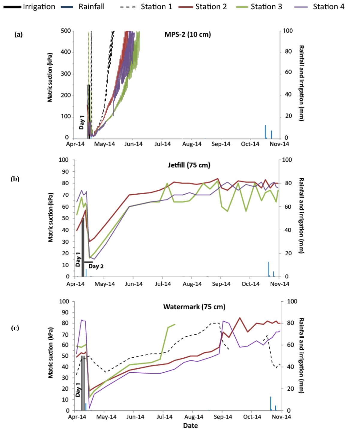
Figure 4.7 : Measured matric suction at depths (a) 10 cm with MPS-2 (only values < 500 kPa are presented due to sensors precision), (b) 75 cm with Jetfill tensiometers and (c) 75 cm with Watermark sensors after the first wetting event
