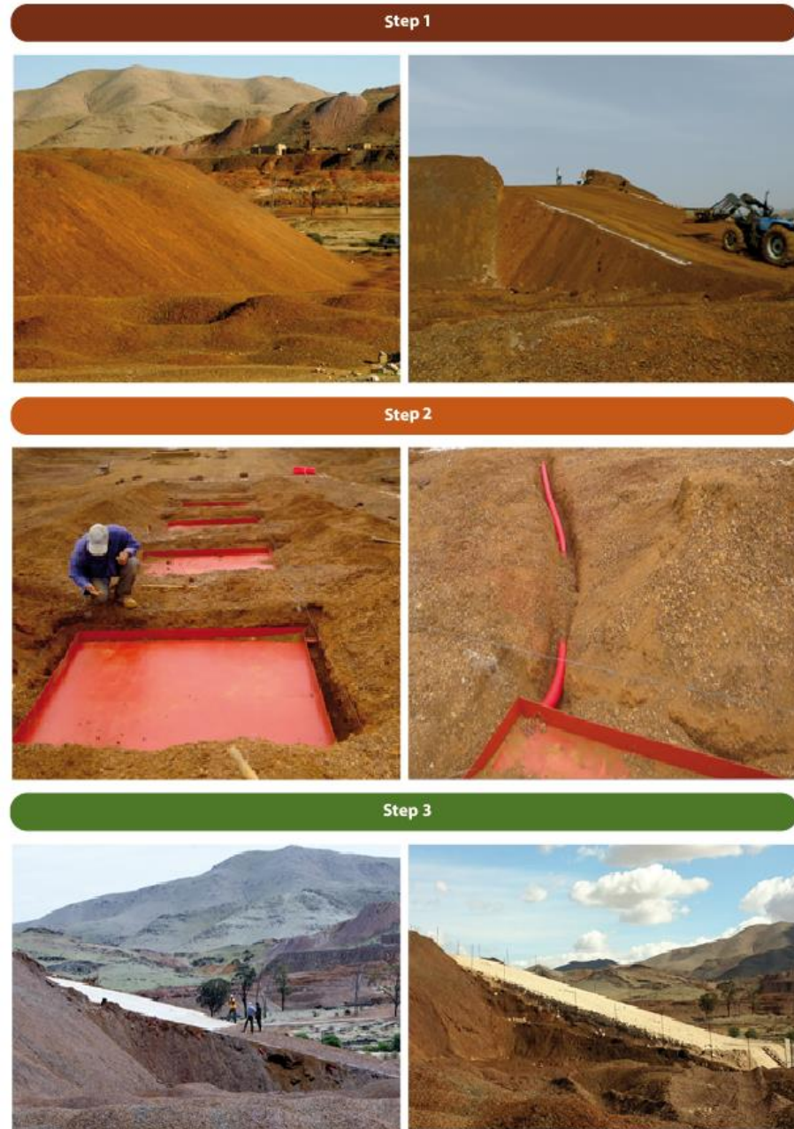
Figure 4.2 : Photos illustrating the inclined SR field experimental cell construction steps Step 1: flattening of the dyke slope; Step 2: installation of the lysimeters; Step 3: placement and compaction of the phosphate mine wastes.
