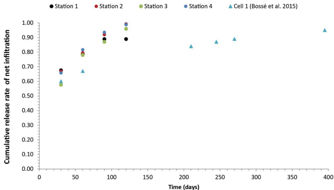
Figure 4.11 : Cumulative release rate of net infiltration evolution after the significant artificial rainfall event simulation (155mm/48)
