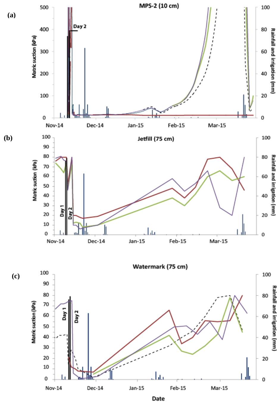
Figure 4.9 : Measured matric suction at depths of (a) 10 cm with MPS-2 ((only values < 500 kPa are presented due to sensors precision), (b) 75 cm with Jetfill tensiometers and (c) 75 cm with Watermark sensors after the second artificial rainfall event reinforced by another natural rainfall event
