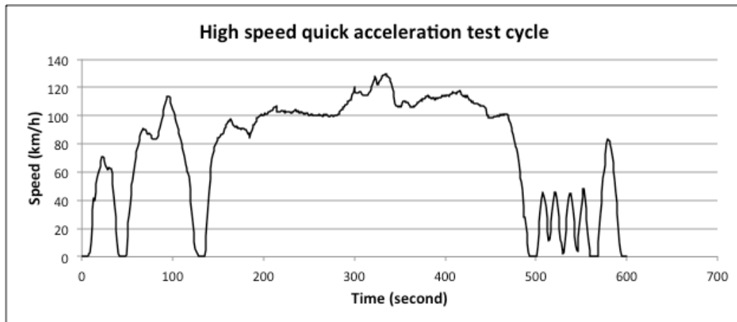
Figure 2.8: The high speed/ quick acceleration test drive cycle (USEPA, 2015)
