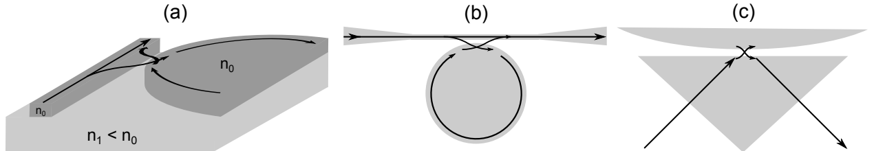
Figure 2.1 : Different coupling configurations - (a) Integrated waveguide and disk (b) Tapered optical fiber (c) Total internal reflection in a prism.
