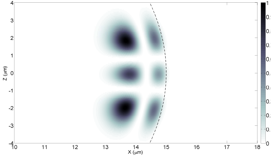
Figure 2.9 : Spatial distribution of TE solutions |\mathbf{e}_j|^2 for an \text{As}_2\text{S}_3 sphere with a radius of 15 \mu\text{m} . The wavelength is 1547 \text{ nm} , l_j = 132 and m_j = l_j - 2 . The dashed line is the cavity's boundary.
