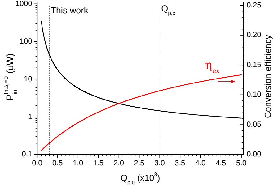
Figure 7.2 : Consequence of a larger intrinsic Q_{p,0} for the pump mode. The Raman mode Q -factors remain constant and are based on the results of Chapter 4.
