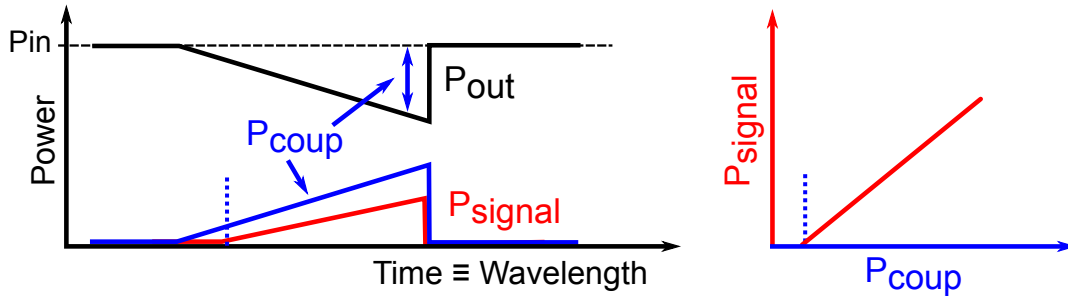
Figure 3.17 : Left plot - Increasing coupled power during thermal drifting. If the coupled power threshold is achieved, the nonlinear or laser signal starts increasing. The constant input power and the threshold are shown as dotted black and blue lines respectively. Right plot - Signal power as a function of the coupled power.
