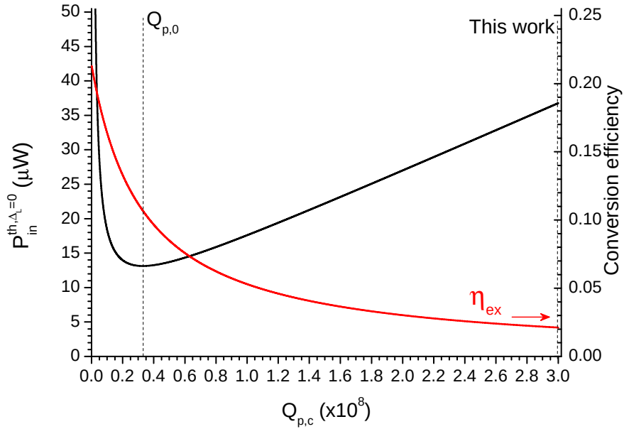
Figure 7.1 : Consequence of a smaller coupling Q-factor Q_{p,c} for the pump mode. The Raman mode Q-factors remain constant and are based on the results of Chapter 4.
