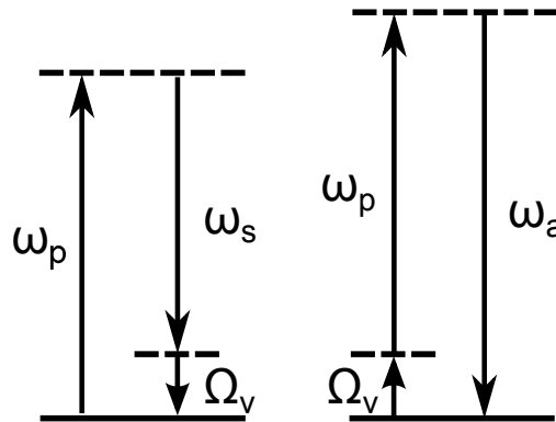
Figure B.4 : Stokes photon \hbar\omega_s and anti-Stokes photon \hbar\omega_a creation through Raman scattering of a pump signal photon \hbar\omega_p .
