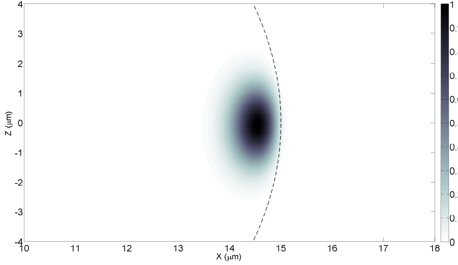
Figure 2.8 : Spatial distribution of TE solutions |\mathbf{e}_j|^2 for an \text{As}_2\text{S}_3 sphere with a radius of 15 \mu\text{m} . The wavelength is 1550 \text{ nm} , l_j = 139 and m_j = l_j . The dashed line is the cavity's boundary.
