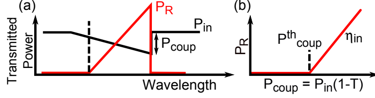
Figure 4.4 : Scheme of the measurements. (a) Oscilloscope view of transmitted pump and Raman emission power P_R . (b) Raman emission power against coupled pump power P_{coup} gives the coupled pump threshold power P_{coup}^{th} and the internal conversion efficiency \eta_{in} of the Raman process. P_{in} and T are the input pump power and the transmission value respectively.
