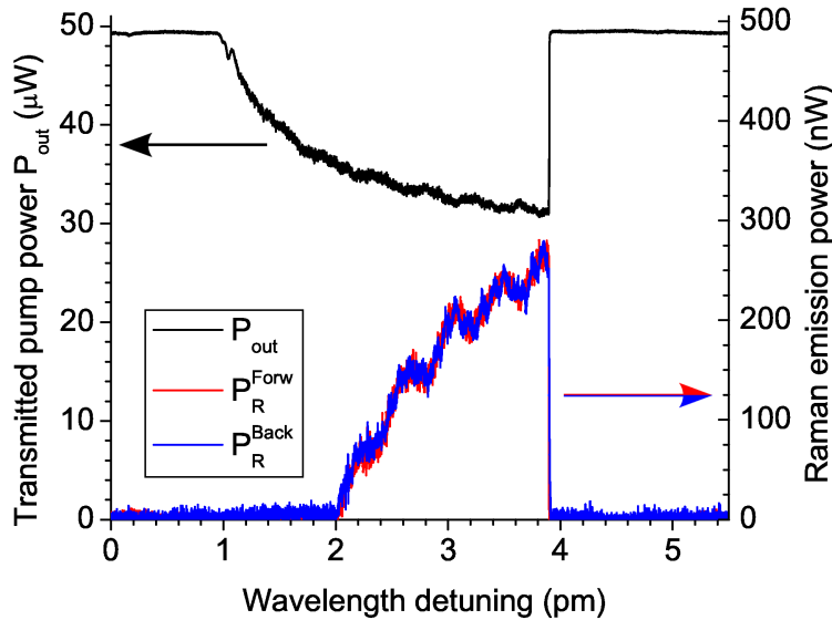
Figure 4.5 : Temporal domain measurements of SRS emission for an input pump power of 49 \mu W with transmitted pump power in black, forward Raman emission in red and backward Raman emission in blue. Raman lasing starts at a detuning of 2 pm.
