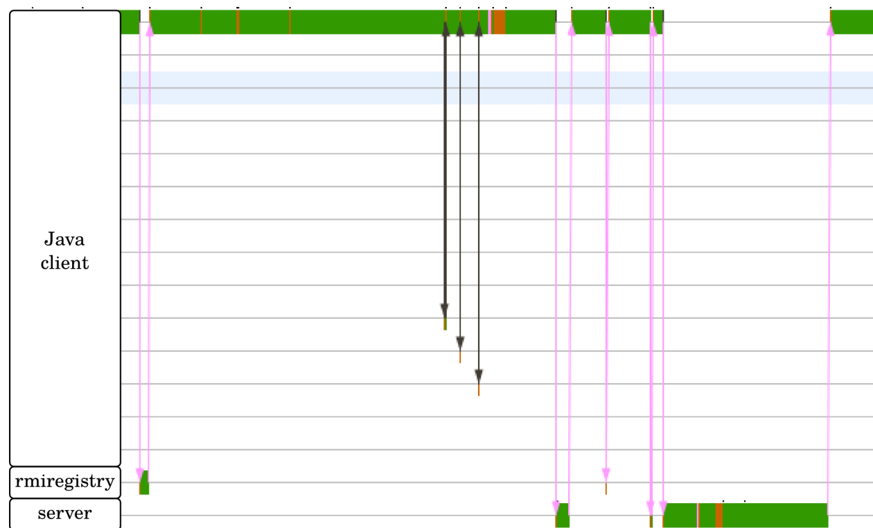
Figure 5.6 Example of Java RMI compute engine execution.
