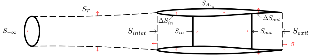
Figure 5.1 Isolated nacelle geometry and surfaces
