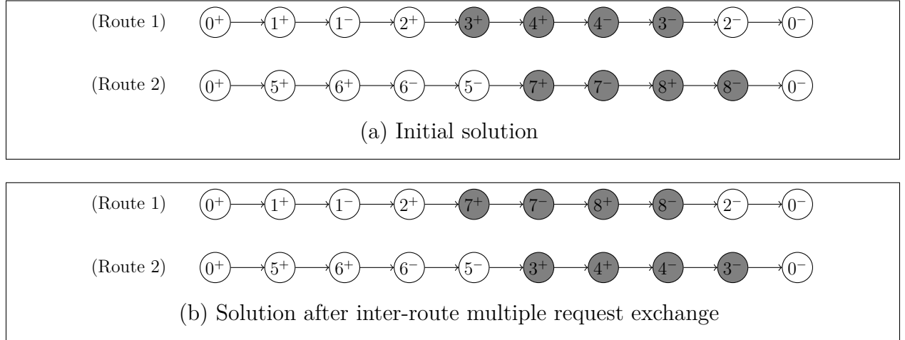
Figure 5.7 – Inter-route multiple request exchange operator : we wish to exchange paths (3^+, 4^+, 4^-, 3^-) and (7^+, 7^-, 8^+, 8^-)
