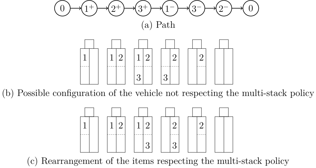
Figure 6.4 – Path for which a possible rearrangement of the items can be found such that the multi-stack policy is respected, q_1 = q_2 = q_3 = 1 and Q = 2
