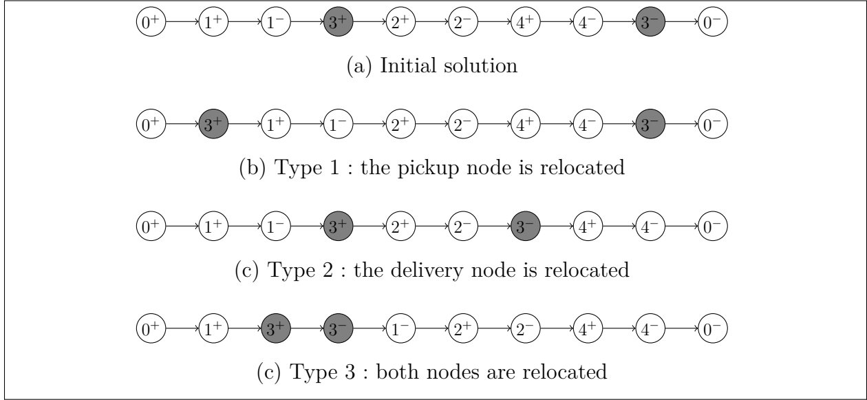
Figure 5.10 – Intra-route request relocate operator : possible relocations of request 3
