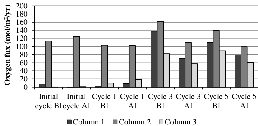
Figure 4.7: Stationary oxygen flux at the base of the tested CCBE based on calculations using a moisture-retaining layer thickness of 0.60 \text{ m} and the corresponding calculated \overline{D_e} .
