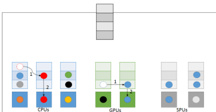
Figure 2-3 Algorithme de Work Stealing
