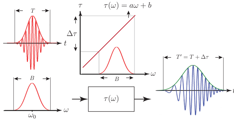
Figure 5.2 Pulse spreading due to dispersion in a conventional phaser. The figure shows the case of a phaser with a linear group delay, but the concept of pulse spreading holds for phasers with more complex responses.
