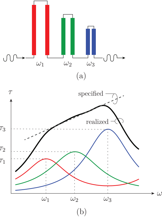
Figure 2.4 Principles of the C-section phaser. (a) Three Cascaded C-section elements [Fig. 2.3(g)] with different lengths. (b) Group delay response formation for (a). Figure has been reproduced from [1].
