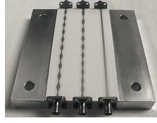
(b) chirped microstrip line [22]
