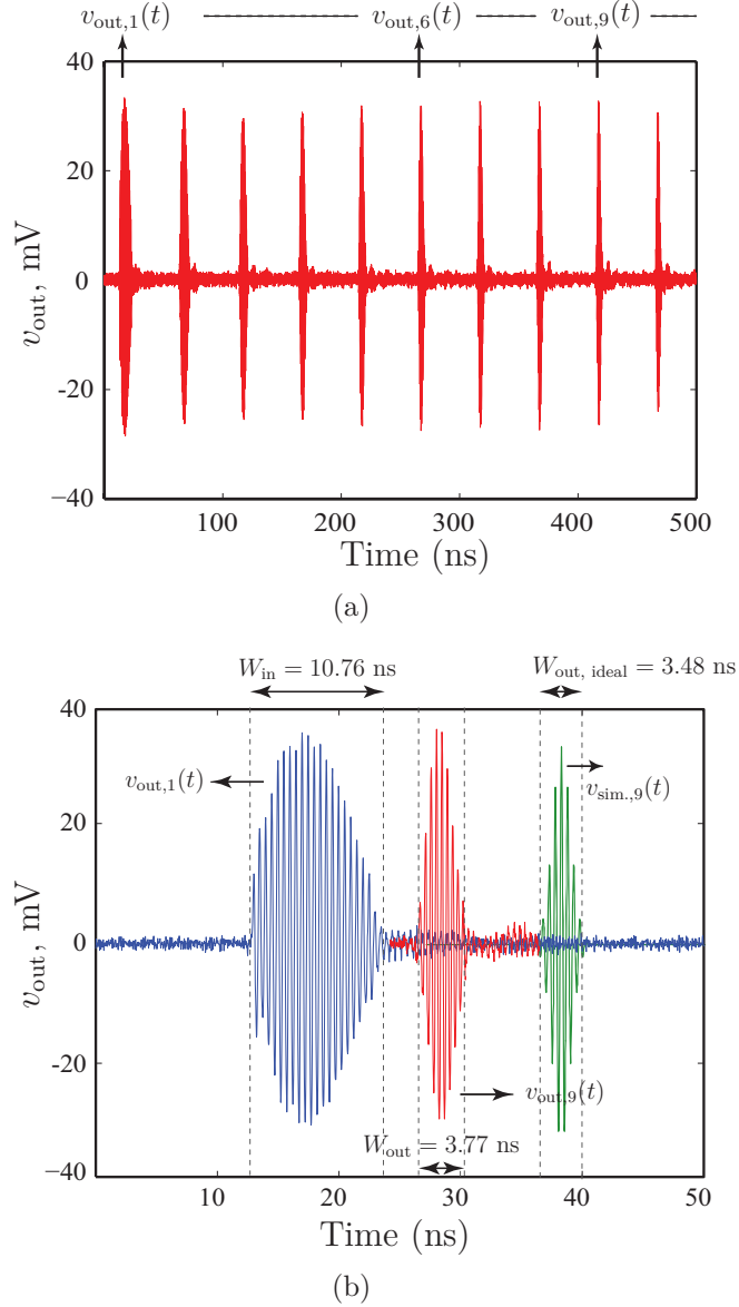
Figure 4.3 Experimental results for the compressor of Fig. 4.2. (a) Output signal v_{out}(t) . (b) Comparison of the first and the 9th output pulses showing an expected pulse width compression by a factor of 2.85. f_{LO} = 2 GHz. v_{sim.,9}(t) is simulated output using (4.2), which has been intentionally shifted by 10 ns for comparison, and v_{out,9}(t) is the measured output result.
