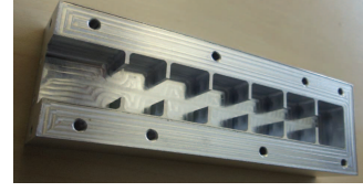
(c) coupled-resonator structure [23]
