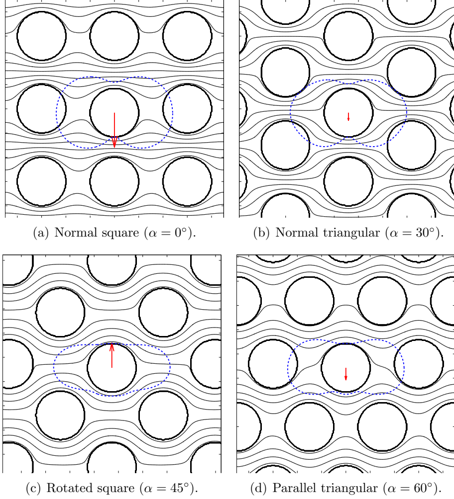
Figure 3.11 Potential flow streamlines and pressure distribution ( -- ) around the central cylinder for the four typical configurations. Central tube was displaced by 8\%D downward while the fluid flows from left to right. The red arrow depicts the resultant lift force.
