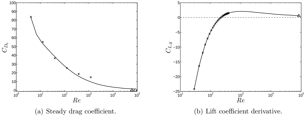
Figure 3.16 Reynolds number-wise interpolation of C_{D_0} and C_{L,y} . Legend: \times : present experiments; \triangle : Shahriary et al. (2007), \circ : Sawadogo and Mureithi (2014b), - : fitting
