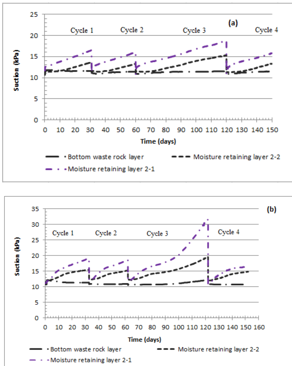
Figure 4-6 : Matric suction measured with MPS-2 sensors installed in different layers of (a) column 1; and (b) column 2.
