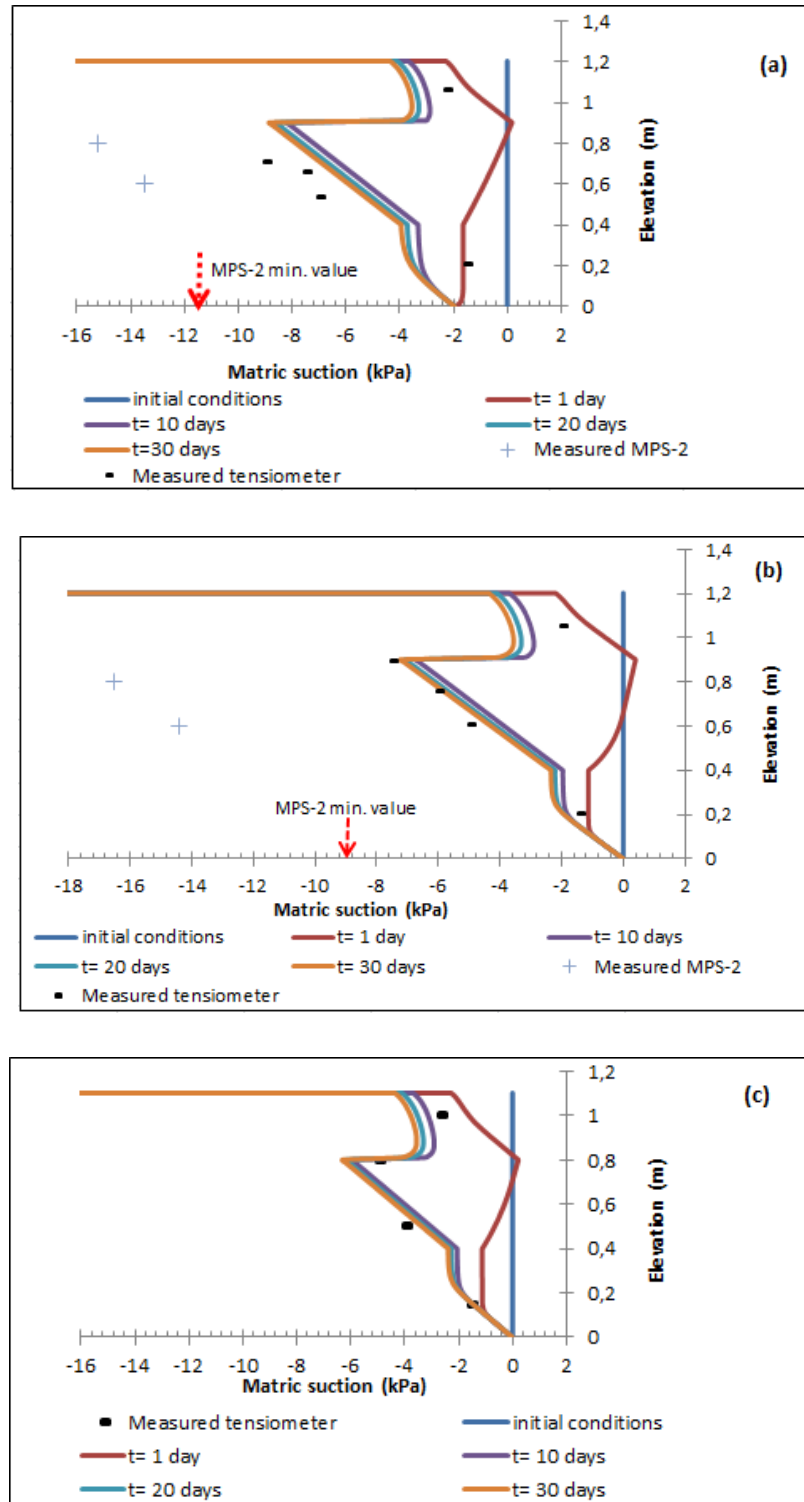
Figure 4-12 : Matric suction measured and modeled with vadose/W with the water table depth of (a) column 1 (with water table depth of 20 cm under the column) ; (b) column 2; and (3) column
