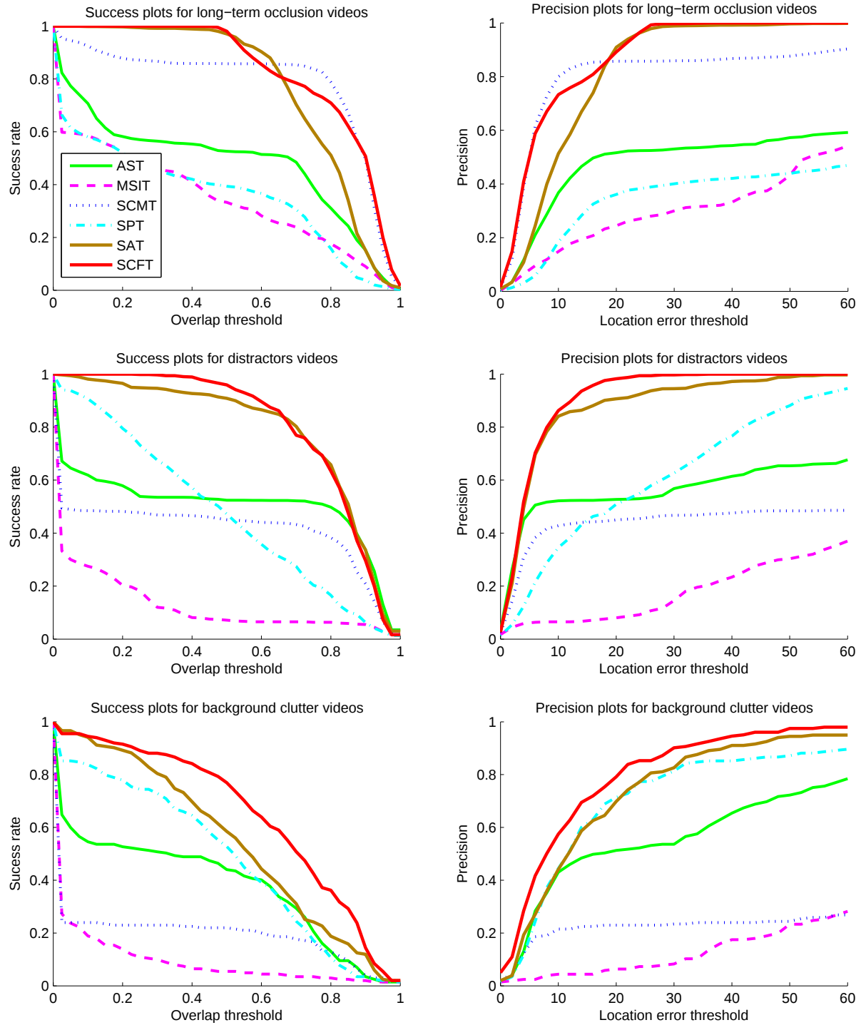
Figure 6.8 Success and precision plots for long-term occlusion, distractors, and background clutter videos.
