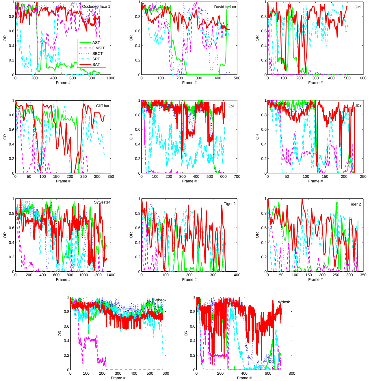
Figure 5.7 Overlap ratio plots.
