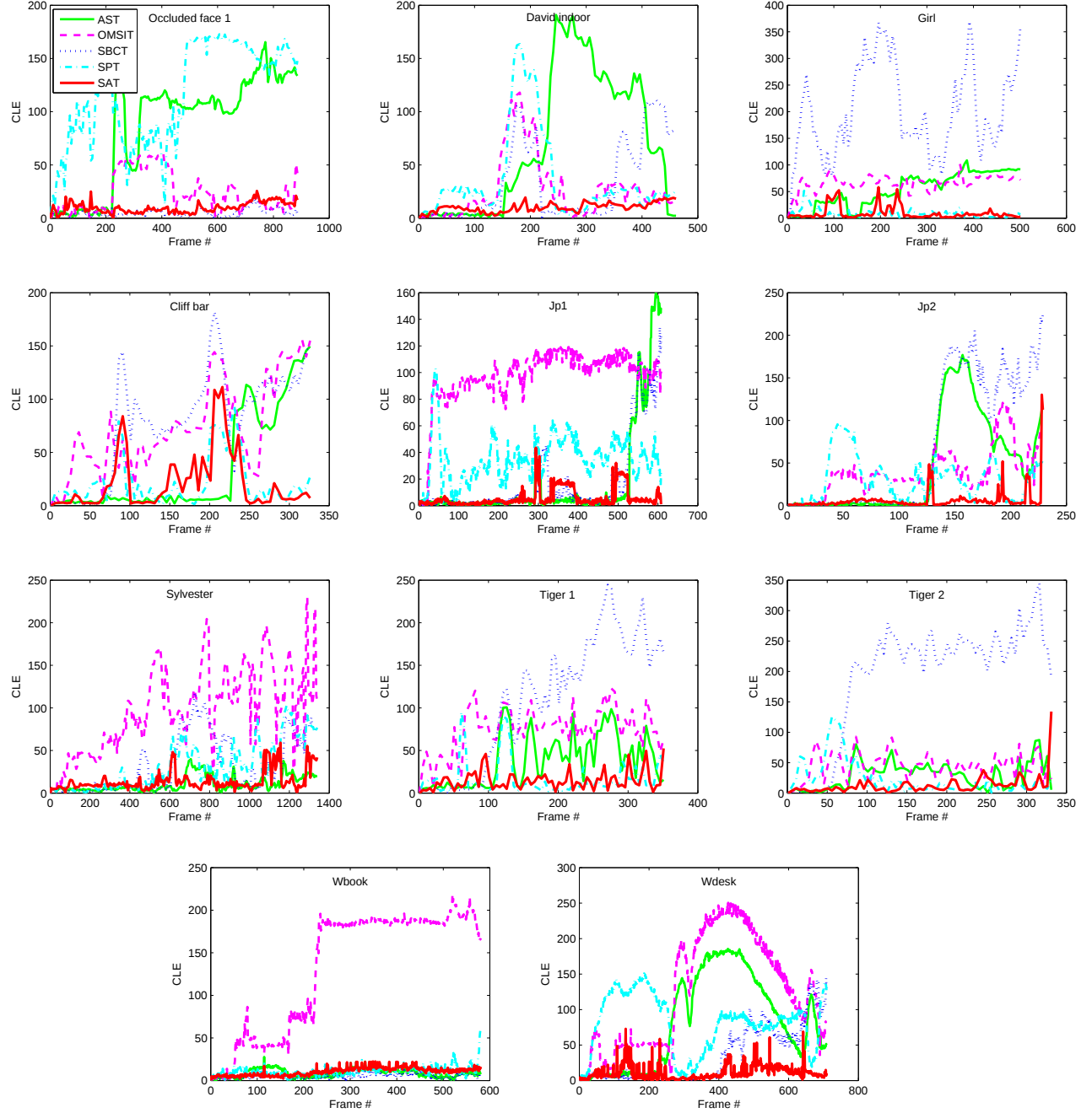
Figure 5.6 Center location error plots.
