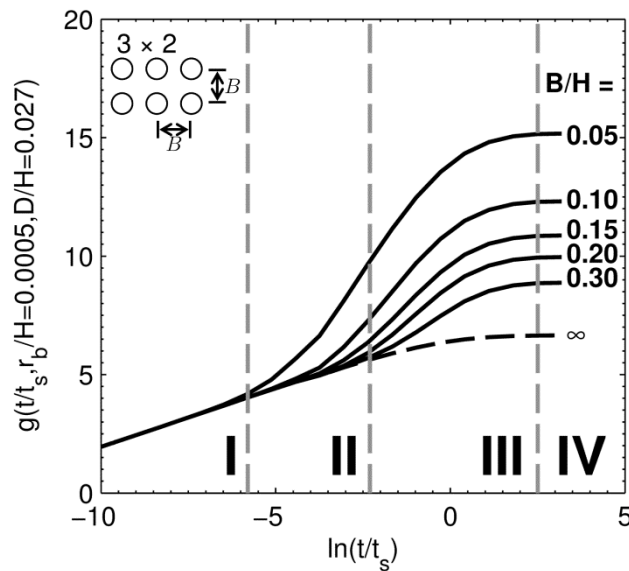
Figure 4-3: Numerical g-functions for a 3 \times 2 bore field
