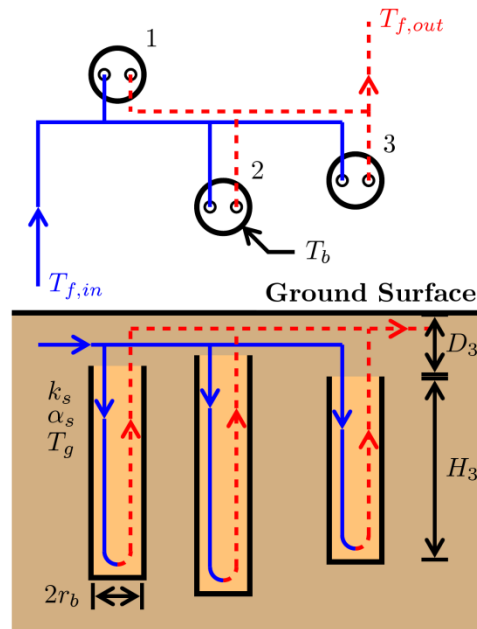
Figure 4-1: Arbitrarily sized and positioned vertical boreholes in an bore field
