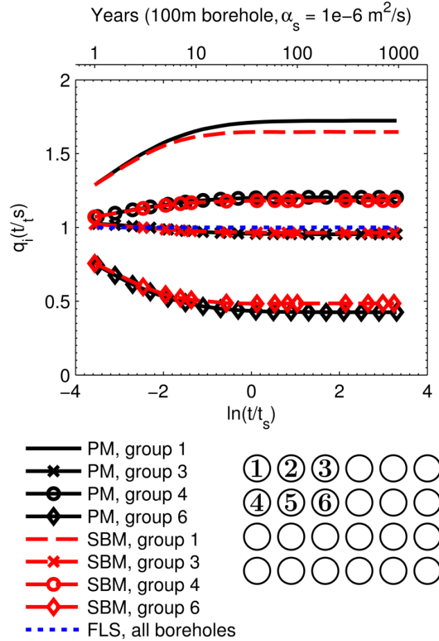
Figure 3-11: Heat extraction rates in a 6 \times 4 bore field, proposed method (PM) and Eskilson's model (SBM)
