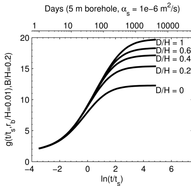
Figure 3-13: g-function of a 6 \times 4 bore field for different buried depth to borehole height ratio obtained with the proposed method
