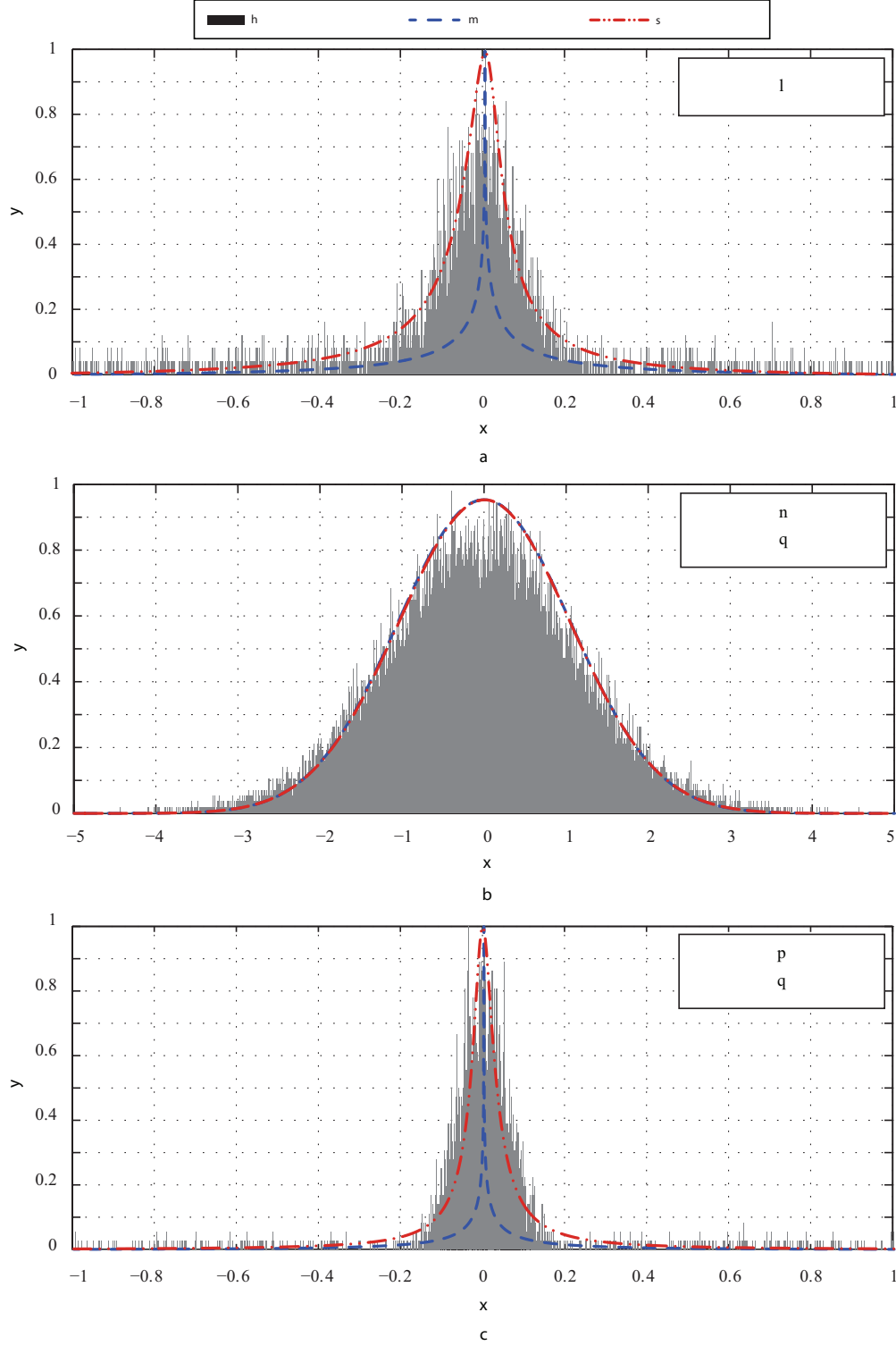
Figure 3.8 A comparison of the empirical interference plus noise signal's pdf with GG and S \alpha S distributions considering different interference channel (a) the AWGN, (b) the residential environment with NLOS link and (c) the open outdoor environment with LOS scenario. N_{cpb} = 32 , N_{burst} = 32 .
