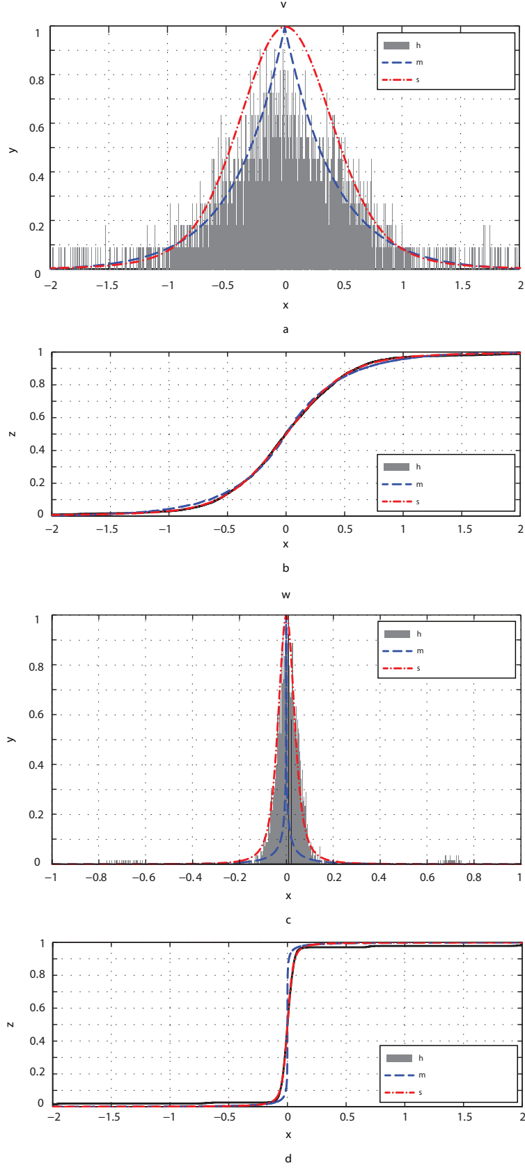
Figure 3.6 A comparison of the pdf and cdf of the interference plus noise signal with GGD and SaS distributions (a) and (b) for INR = 0dB, (c) and (d) for INR = 20dB, respectively.
