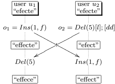
Figure 3.1 Integration without transformation.
