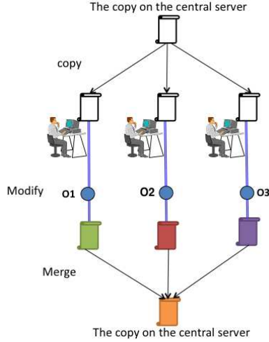
Figure 3.3 MV approach
