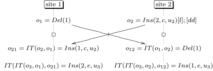
Figure 3.9 Violation of TP2 for Ressel's IT (in case u_2 < u_3 ).
