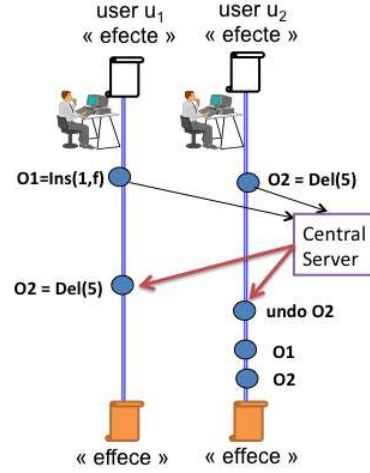
Figure 3.4 SRC approach
