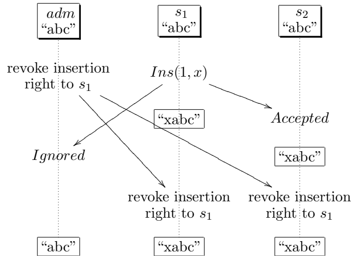
Figure 4.2 Divergence caused by introducing administrative operations
