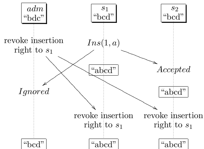
Figure 5.5 Divergence caused by introducing administrative operations
