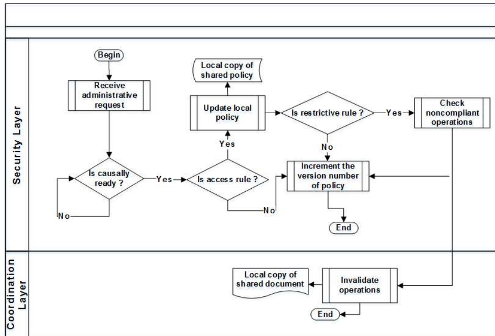
Figure 5.4 Processing of received administrative request.
