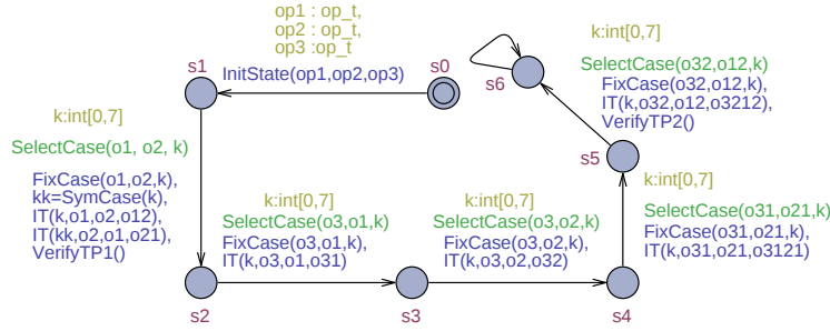
Figure 3.18 Automaton used to verify TP1 and TP2
