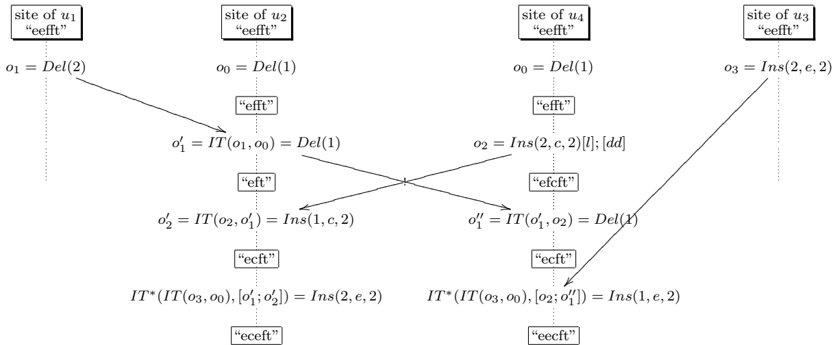
Figure 3.10 Violation of TP2 for Imine's IT.
