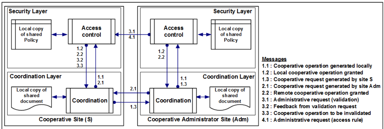
Figure 4.1 Flow of collaboration messages
