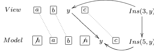
Figure 3.19 View and Model states (Figure taken from [Oster et al. (2006a)]).
