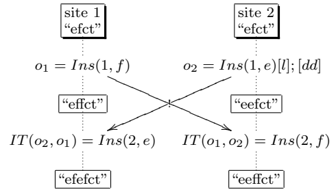
Figure 3.7 Violation of TP1 for Sun's IT.
