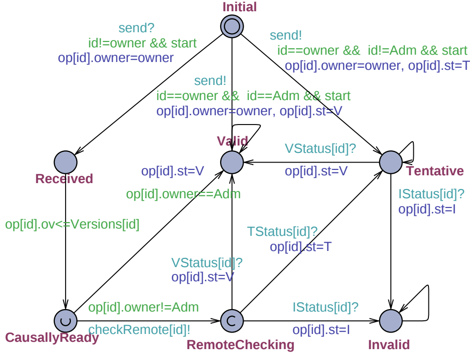
Figure 5.7 The model of cooperative operation.
