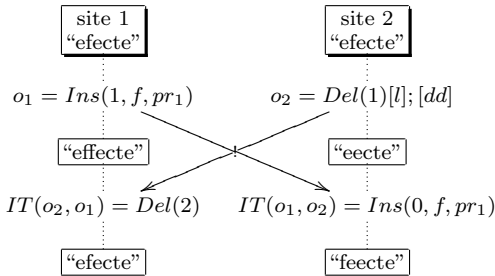
Figure 3.6 Violation of TP1 for Ellis's IT.
