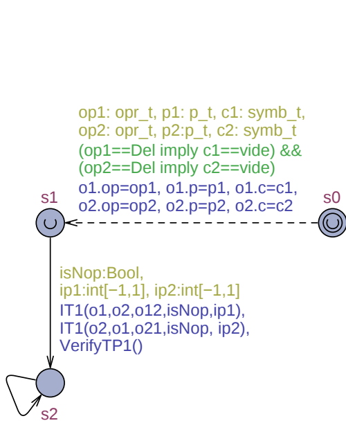
Figure 3.11 Synthesize an IT for TP1
