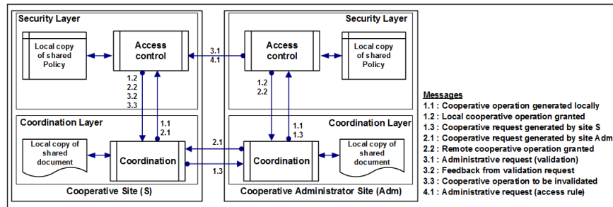
Figure 5.1 Flow of collaboration messages
