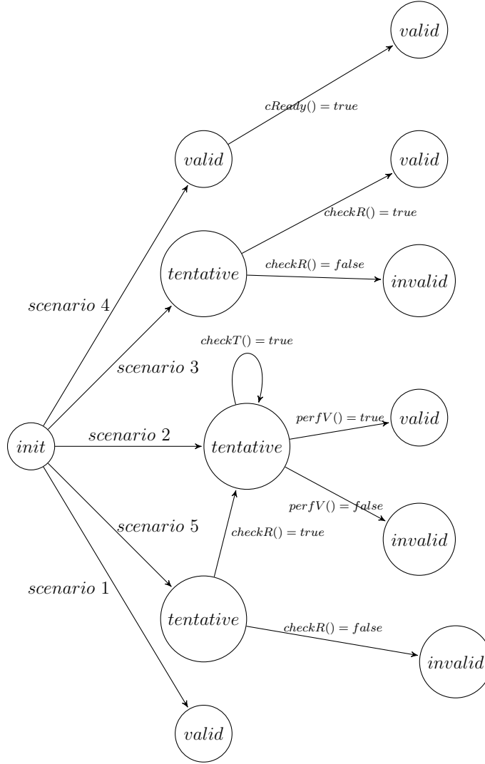
Figure 5.6 Execution process at any site.
