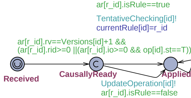
Figure 5.8 The model of administrative request.
