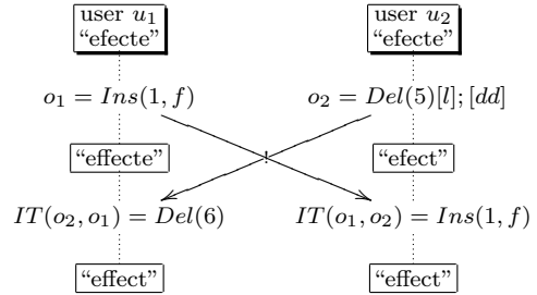
Figure 3.2 Integration with transformation.
