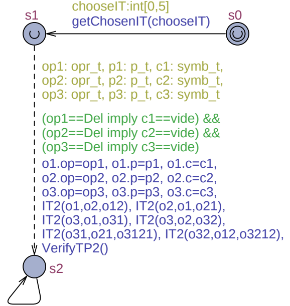
Figure 3.12 Synthesize a consistent IT
