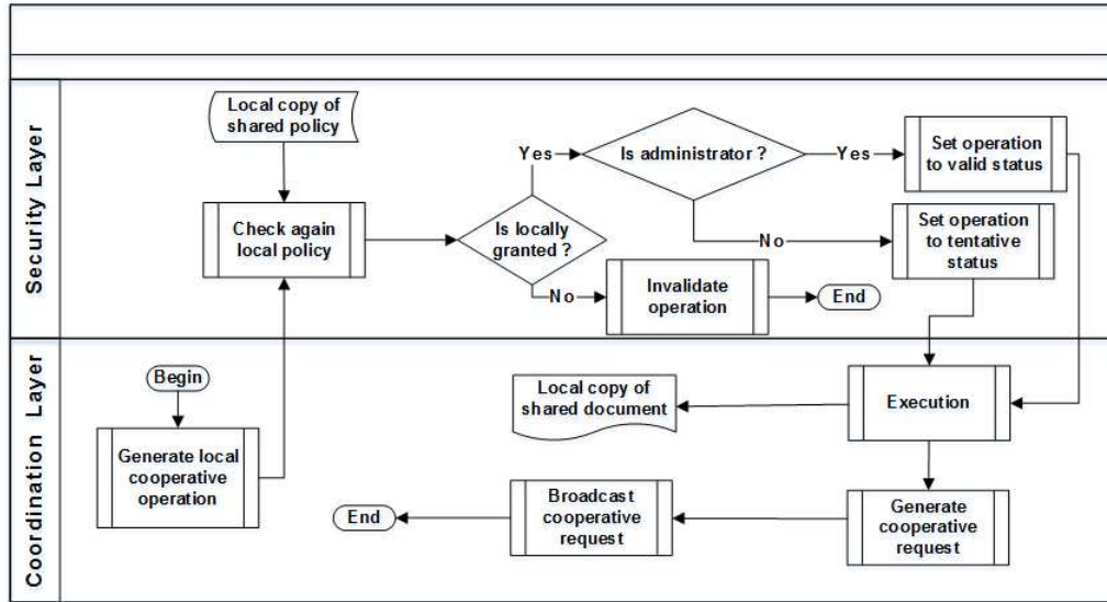
Figure 5.2 Processing of a cooperative operation at generation time.
