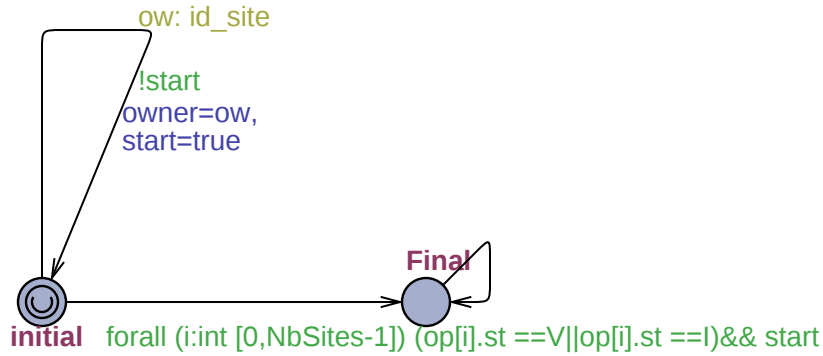
Figure 5.10 Automaton devoted to choose the owner of the cooperative operation.
