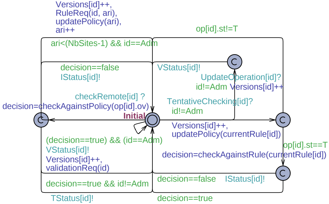
Figure 5.9 The model of ACP.
