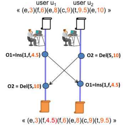
Figure 3.5 CRDT approach
