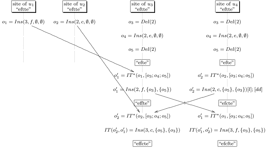
Figure 3.8 Violation of TP1 for Suleiman's IT.
