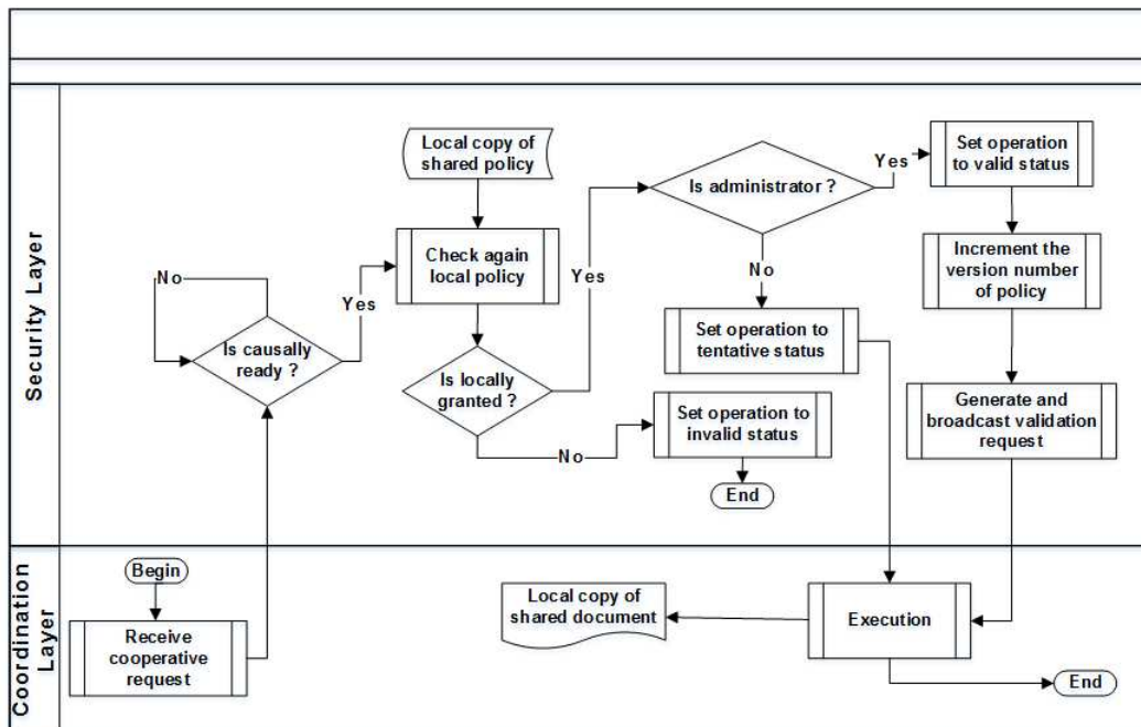
Figure 5.3 Processing of a received cooperative operation.
