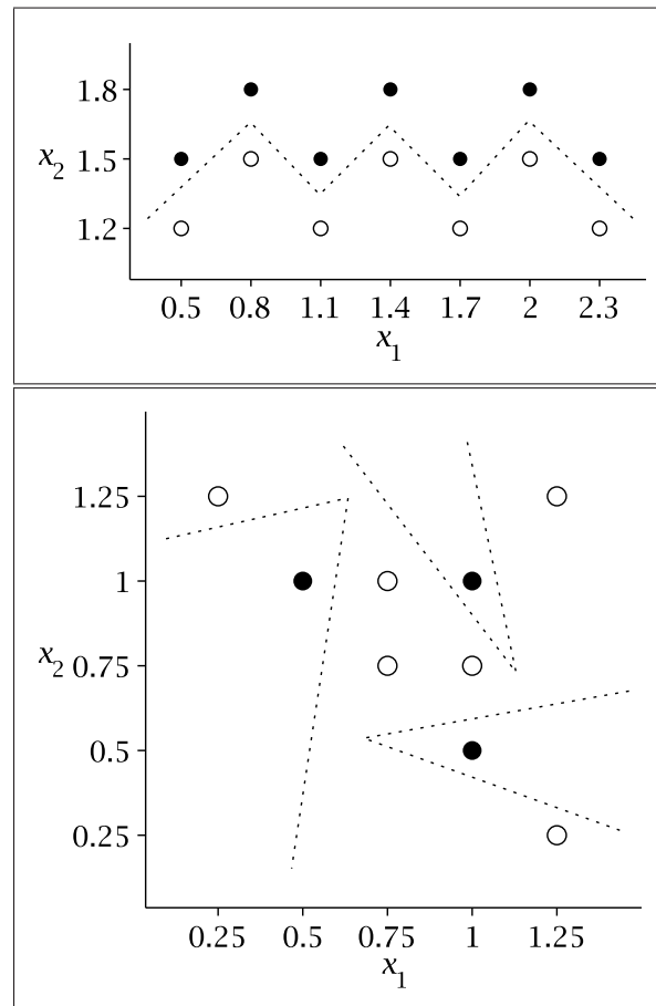
Figure 3.8 Triangular waveform problem (top) and isolated points problem (bottom). White dots (respectively black dots) represent inputs with a desired value of 1 (respectively 0). The dashed lines represent piecewise linear classification boundaries.
