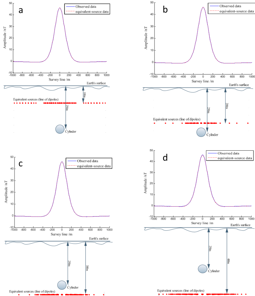
(a) Equivalent-source at the depth of 100m; (b) Equivalent-source at the depth of 200m (c) Equivalent-source at the depth of 300m; (d) Equivalent-source at the depth of 400m
