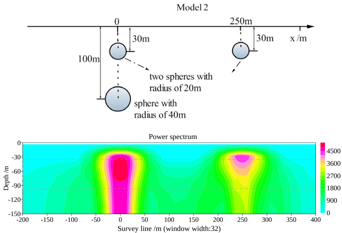
(a) Depth image with the window width of 32
