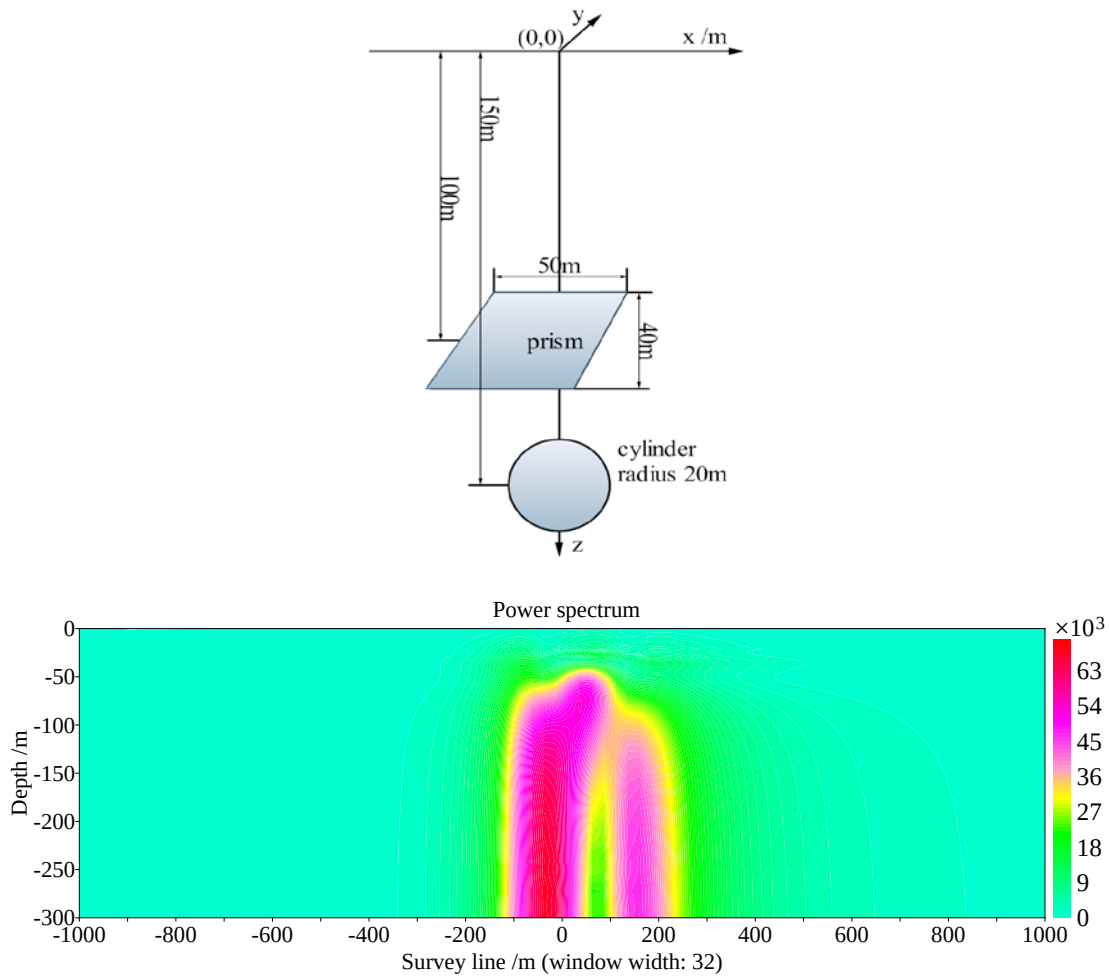
(a) Depth image with the window width of 32
