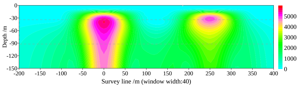
(b) Depth image with the window width of 40
