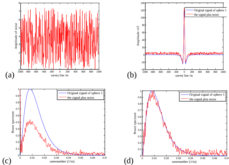
Figure 2.11: NSR=3%, (a) Random noise (NSR=3%), (b) original signal and the signal plus noise, (c) power spectrum and (d) power spectrum with DC component removed of shallow sphere 1
