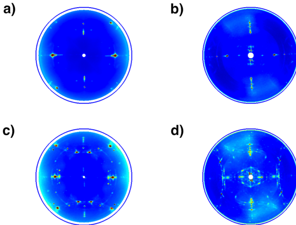
Figure 4.19 MnP (020) pole figures of a) MnP-600-15 and b) MnP-650-15, as well as MnP (111) pole figures of c) MnP-600-15 and d) MnP-650-15. We observe more features on the pole figures of MnP-650-15 than MnP-600-15. The pole figures have been obtained using a linear detector.
