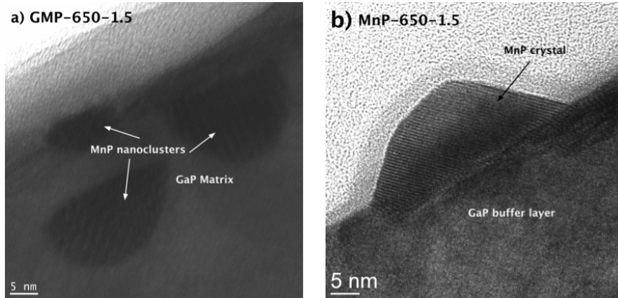
Figure 5.9 a) MnP nanoclusters embedded in GaP (GMP-650-1.5) compared to b) MnP crystal grown endotaxially on GaP (GMP-650-1.5).
