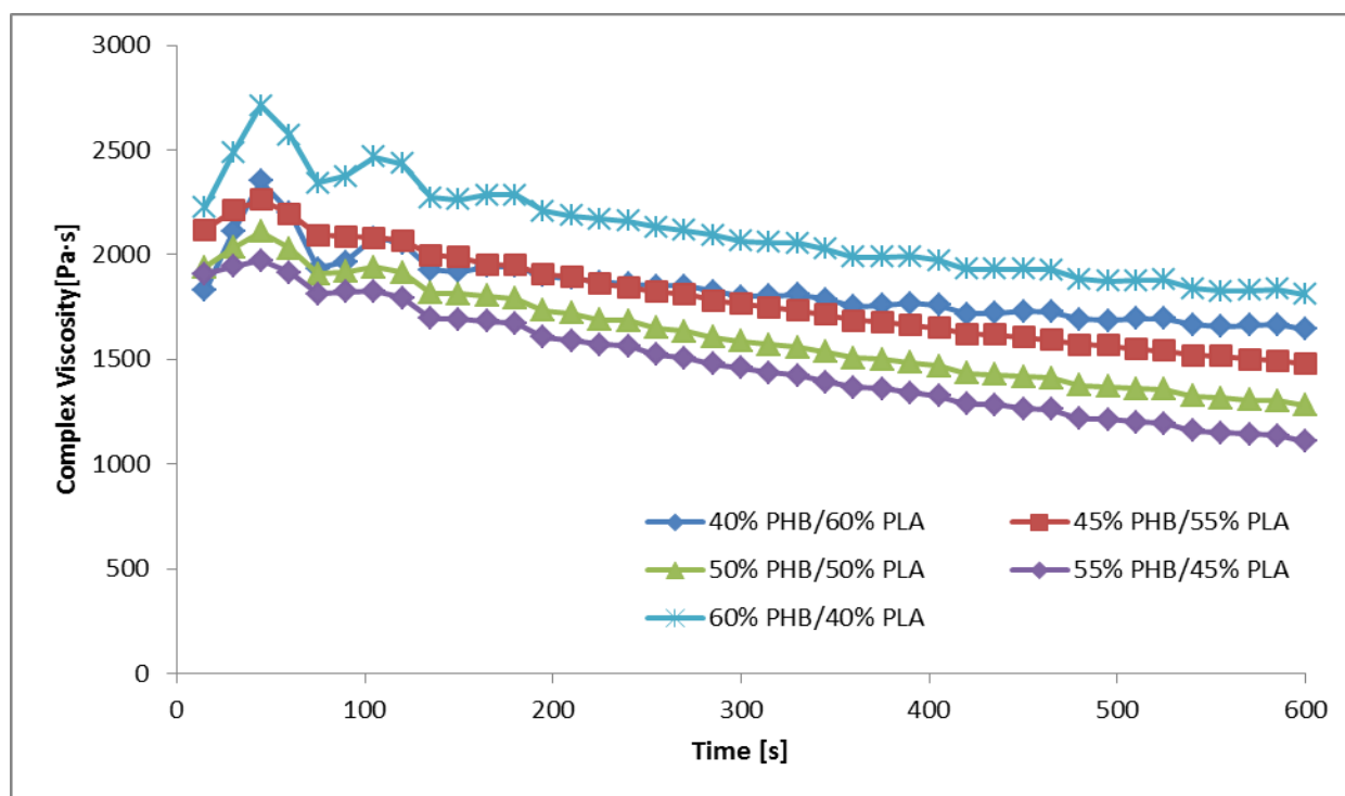
Figure A10: Complex viscosity of PHB/PLA blends in the vicinity of 50% PHB/50% PLA
